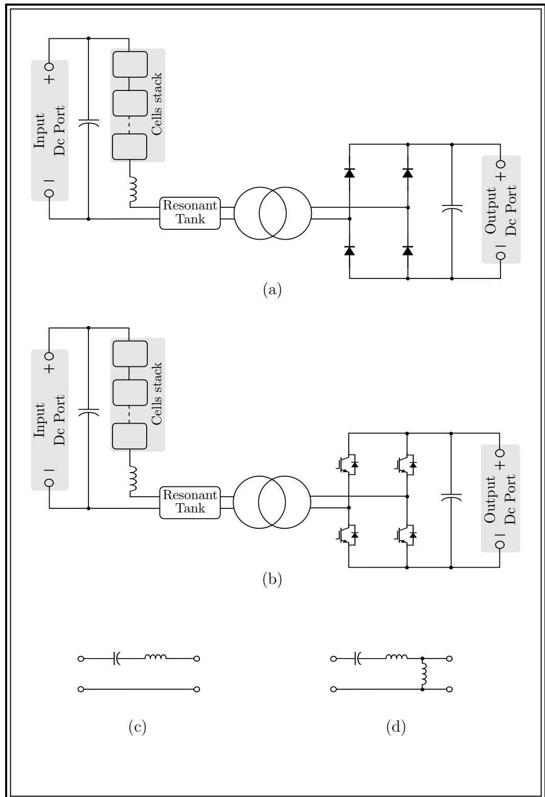
Figure 2.6: Monopole asymmetrical dc-ad-dc resonant MMC: (a) diodes bridge as low voltage ac-dc converter, (b) full-bridge as low voltage ac-dc converter, (c) series LC resonant tank, and (d) LLC resonant tank.
