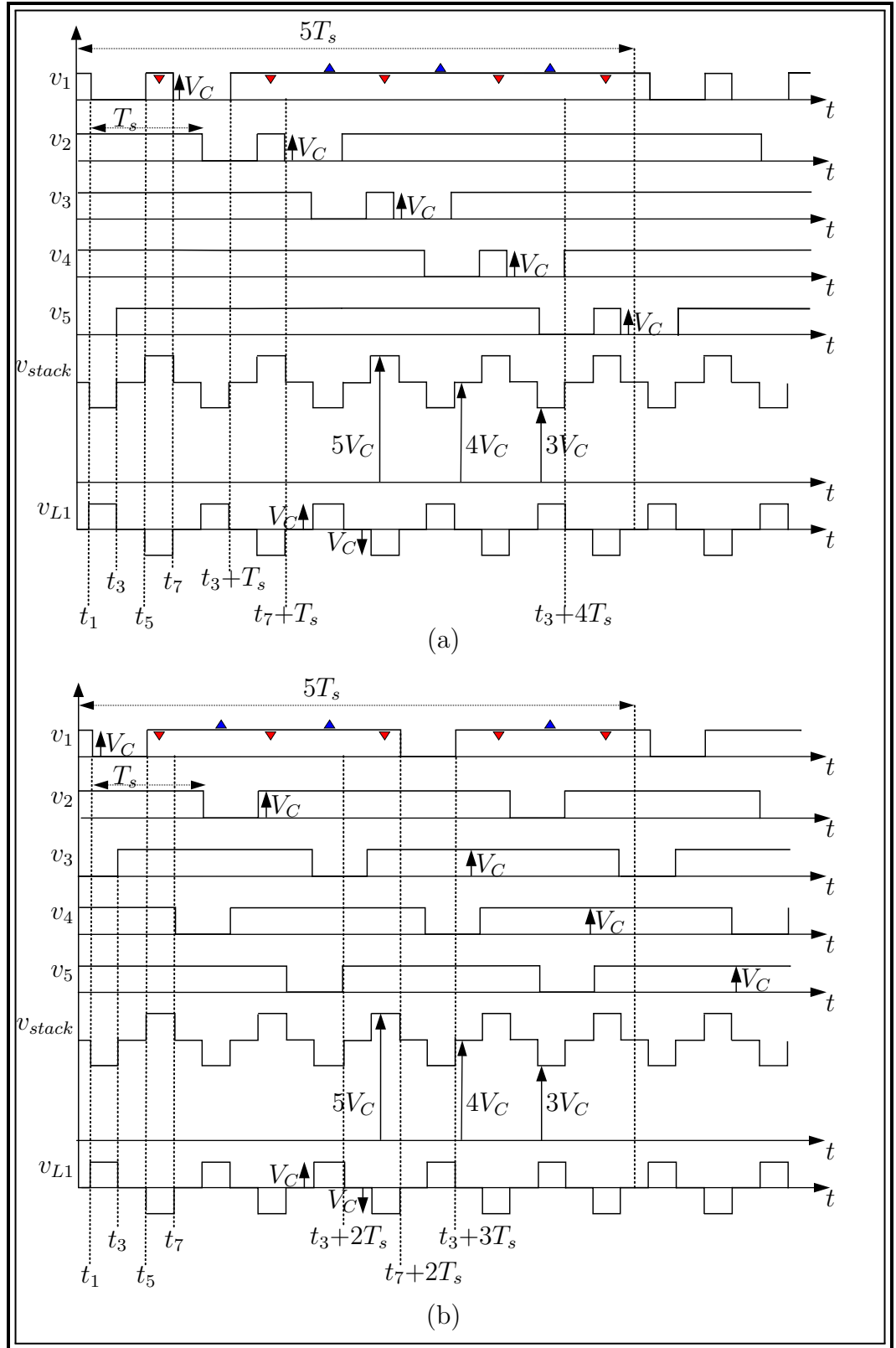
Figure 4.3: Modulation wave-forms in the stack of five cells in the period 5T_s : (a) case j = 0 , and (b) case j = 2 .
