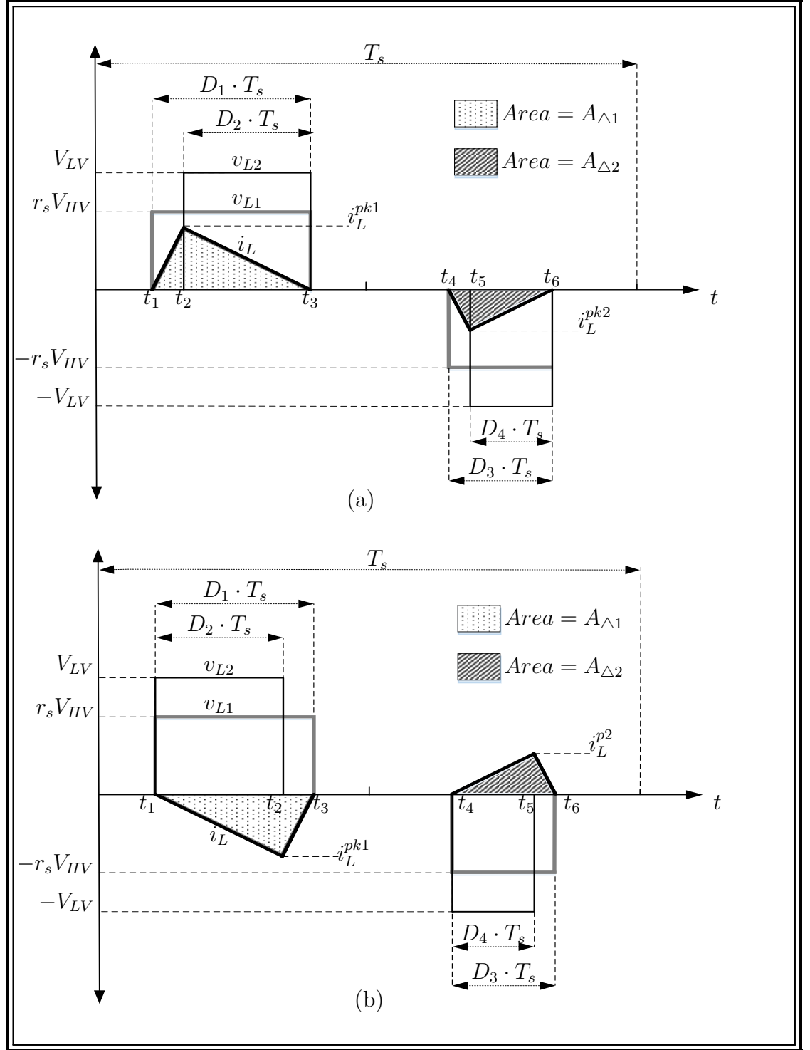
Figure 3.5: Ac-link waveforms under ZCS-ATCM and r_V > 1 : (a) HV to LV power-flow, and (b) LV to HV power-flow.
