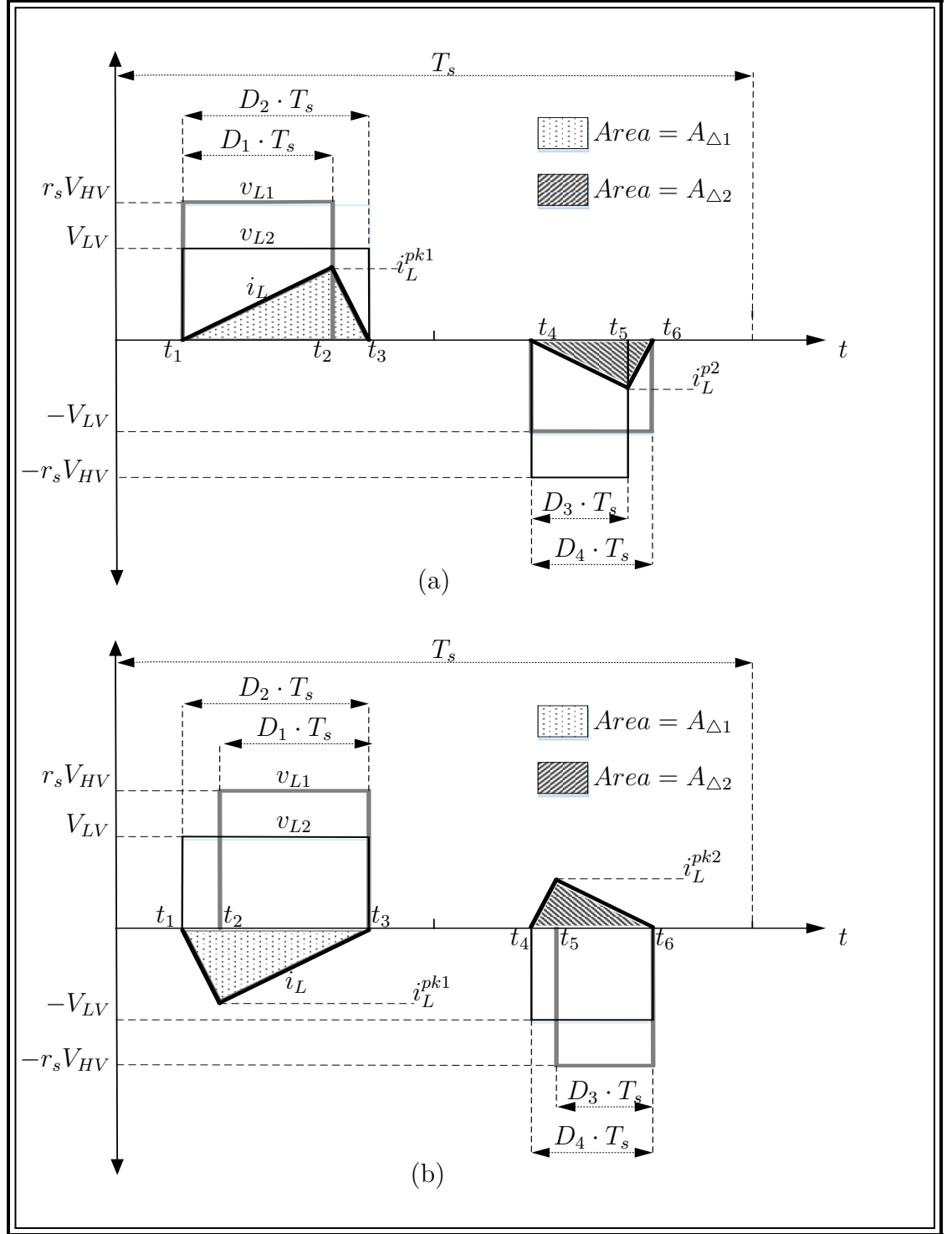
Figure 3.8: Ac-link waveforms under ZCS-ATCM and r_V < 1 (a) HV to LV power-flow, and (b) LV to HV power-flow.
