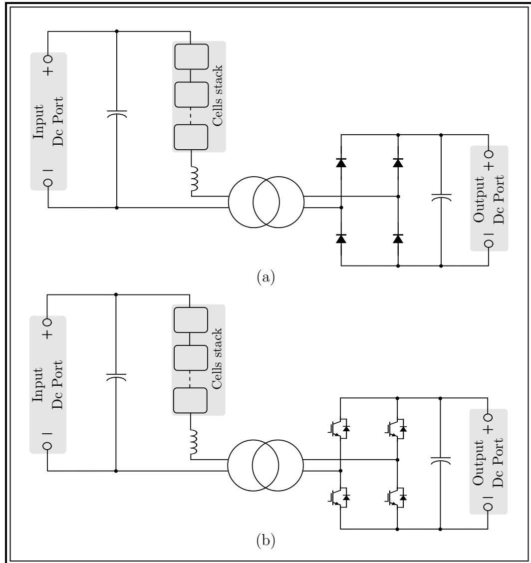
Figure 2.8: Monopole asymmetrical dc-ad-dc MMC: (a) diodes bridge as low voltage ac-dc converter, and (b) full-bridge as low voltage ac-dc converter.
