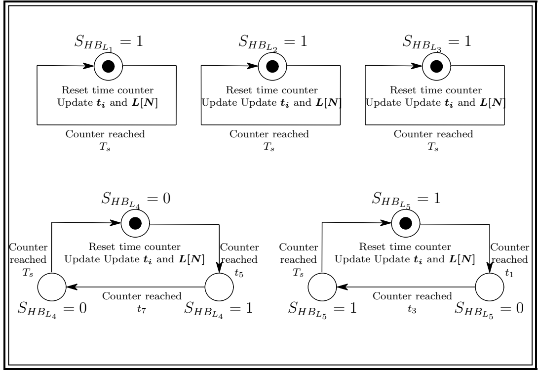
Figure C.2: Half-bridge finite state machines (FSMs) for the case of five cells in the stack and time-controlled sorting modulation.
