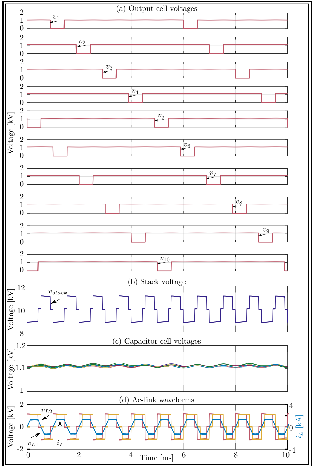
Figure 5.1: Simulation results at full-scale, typical waveforms: (a) Output cell voltages for ten cells using phase-shift modulation, (b) Resulting total stack voltage, (c) MMC capacitor voltages ten cells, and (d) Ac-link inductor voltages and current.
