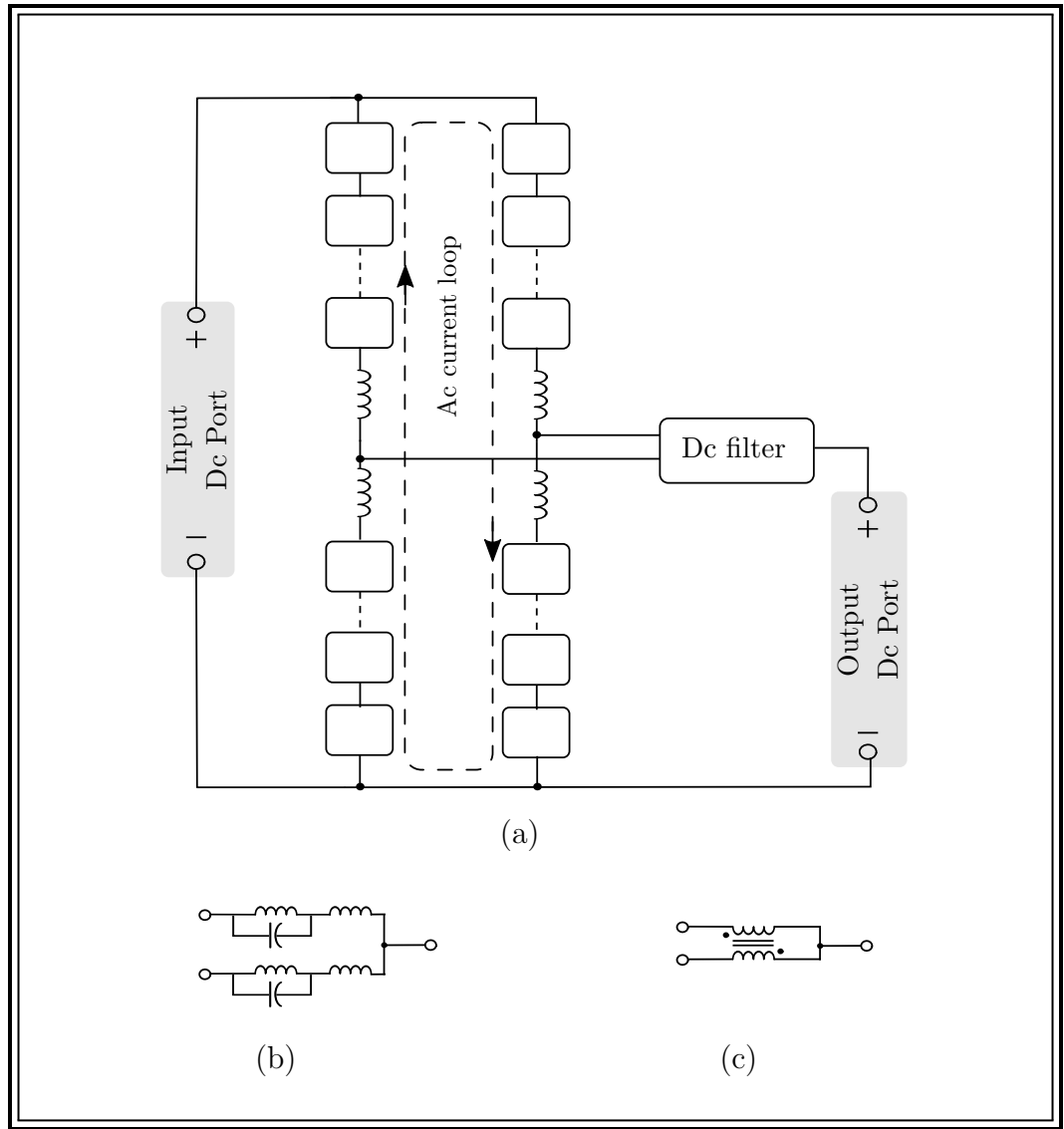
Figure 2.15: Buck-Boost interleaved structure : (a) DC-MMC using two legs (b) Dc filter: passive solution, and (c) Dc filter: coupled inductors.
