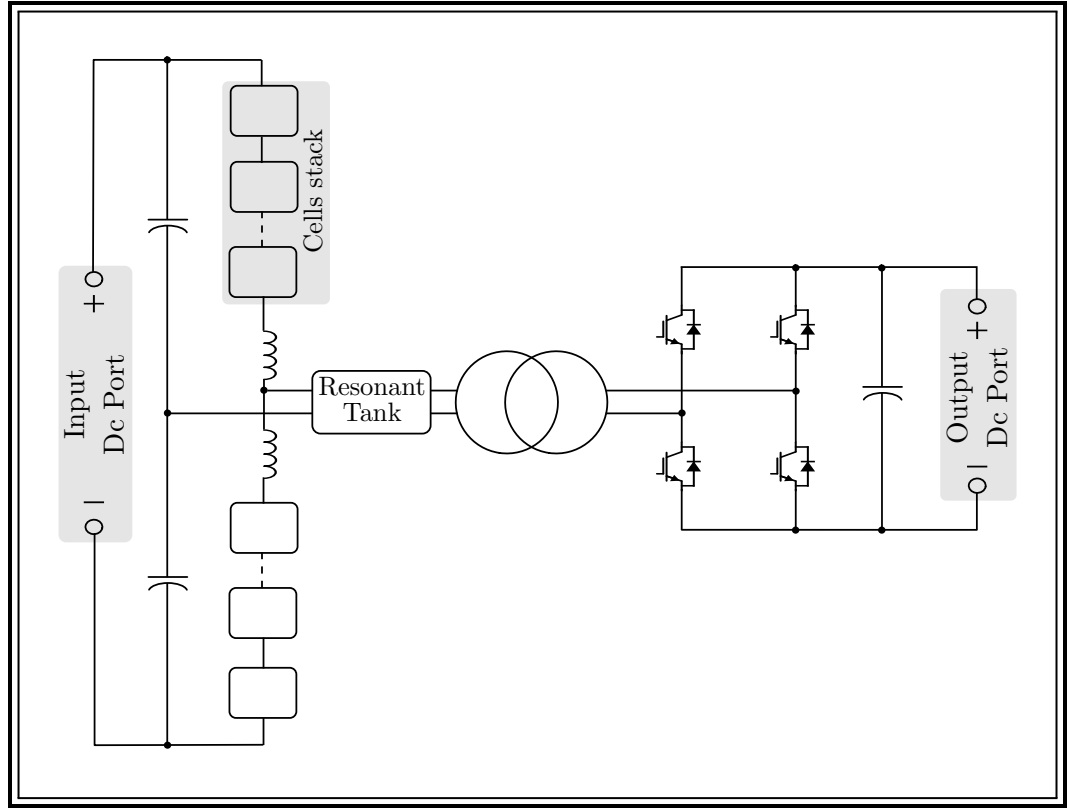
Figure 2.7: Bipole asymmetrical dc-ad-dc resonant MMC using a full-bridge as low voltage ac-dc converter.
