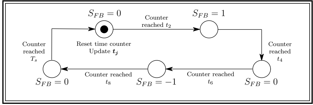
Figure C.3: Full-bridge finite state machine (FSM).
