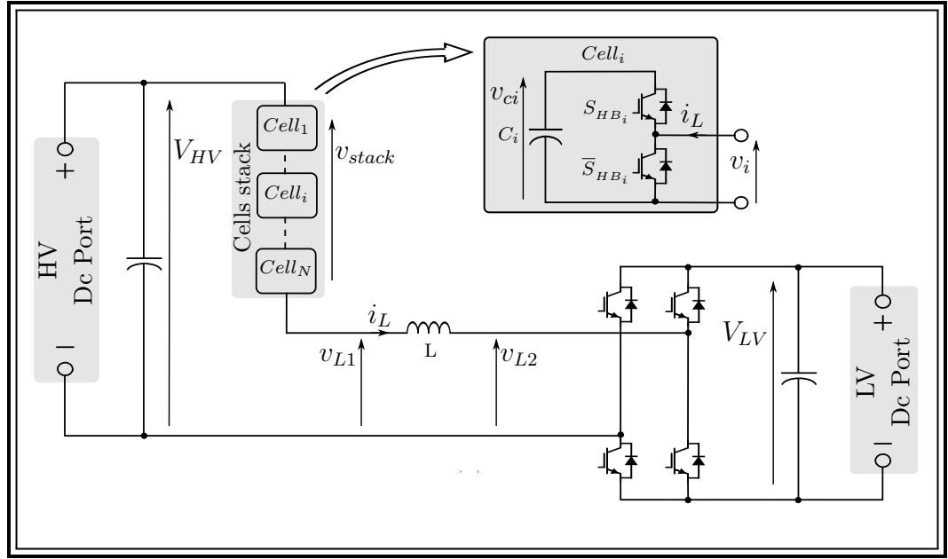
Figure 3.1: High step ratio dc-dc MMC topology.
