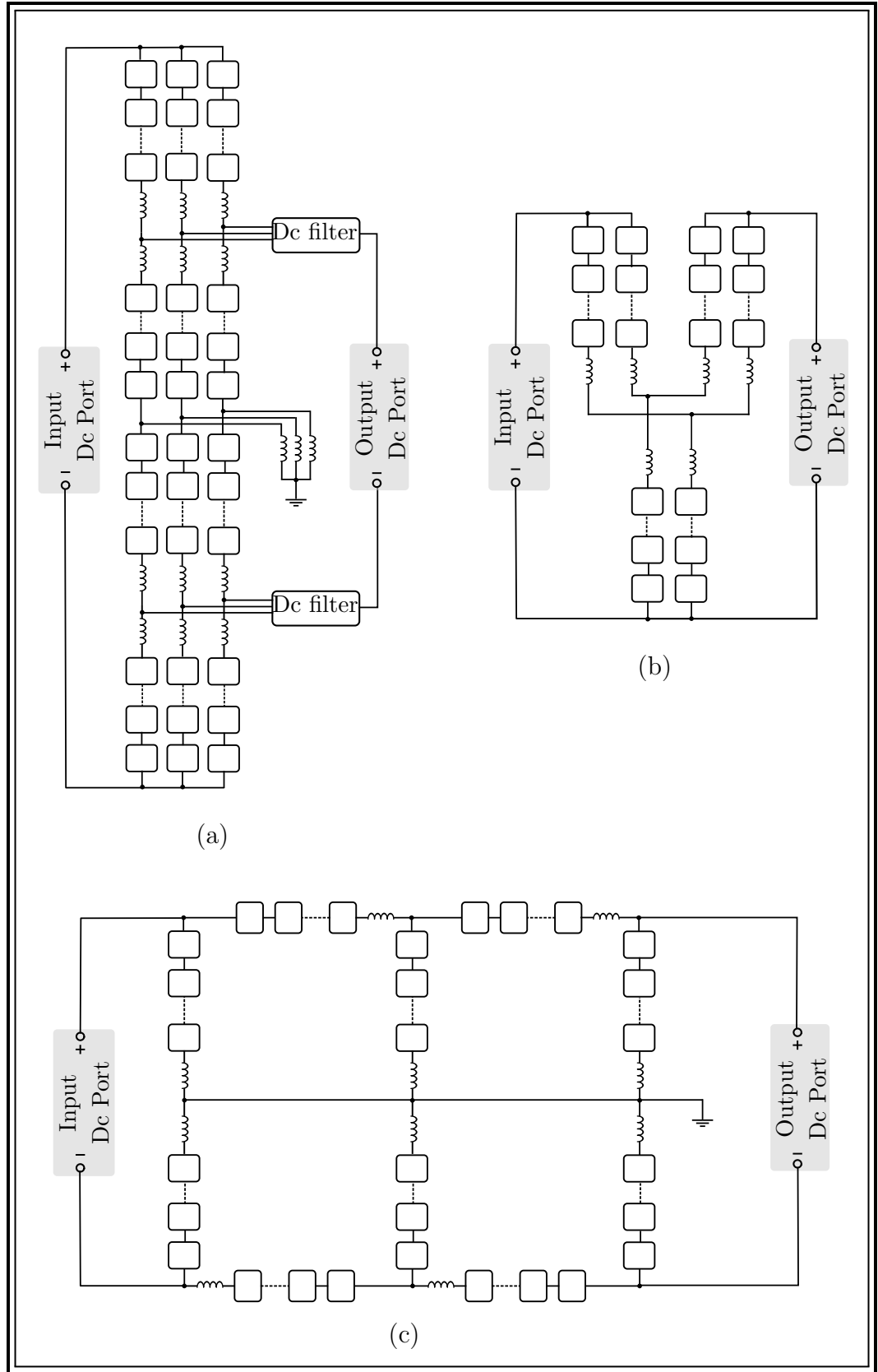
Figure 2.16: DC-MMC derivations : (a) DC-MMC symmetrical monopole configuration (b) Double Wye structure, and (c) Double II structure.
