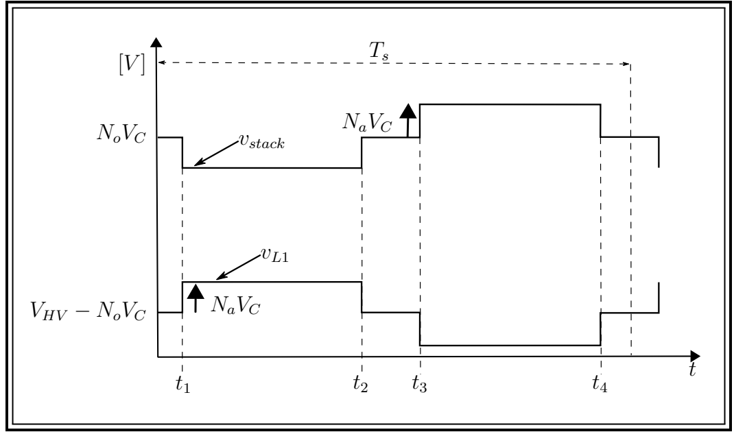
Figure 3.2: General three-level square-waveform stack operation.
