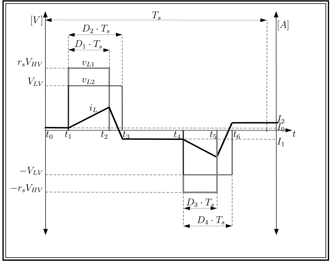
Figure 3.7: General ac-link waveforms for positive power-flow under asymmetrical triangular current mode and r_V < 1 .
