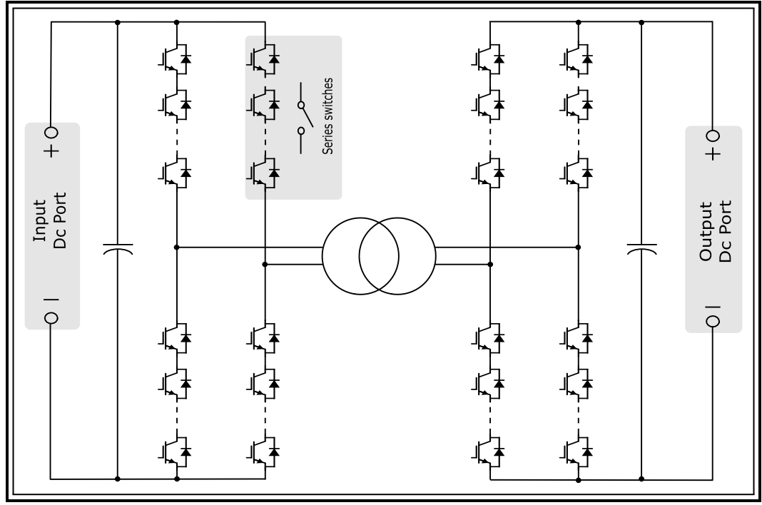
Figure 2.3: Two level dual active bridge using series switches.
