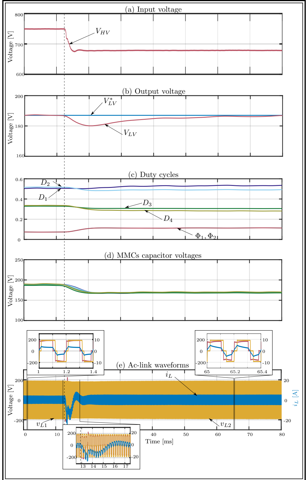
Figure 7.8: Experimental results for V_{HV} step response: (a) Input voltage, (b) Output voltage, (c) Duty cycles, (d) MMC capacitor voltages, and (e) Ac-link waveforms.
