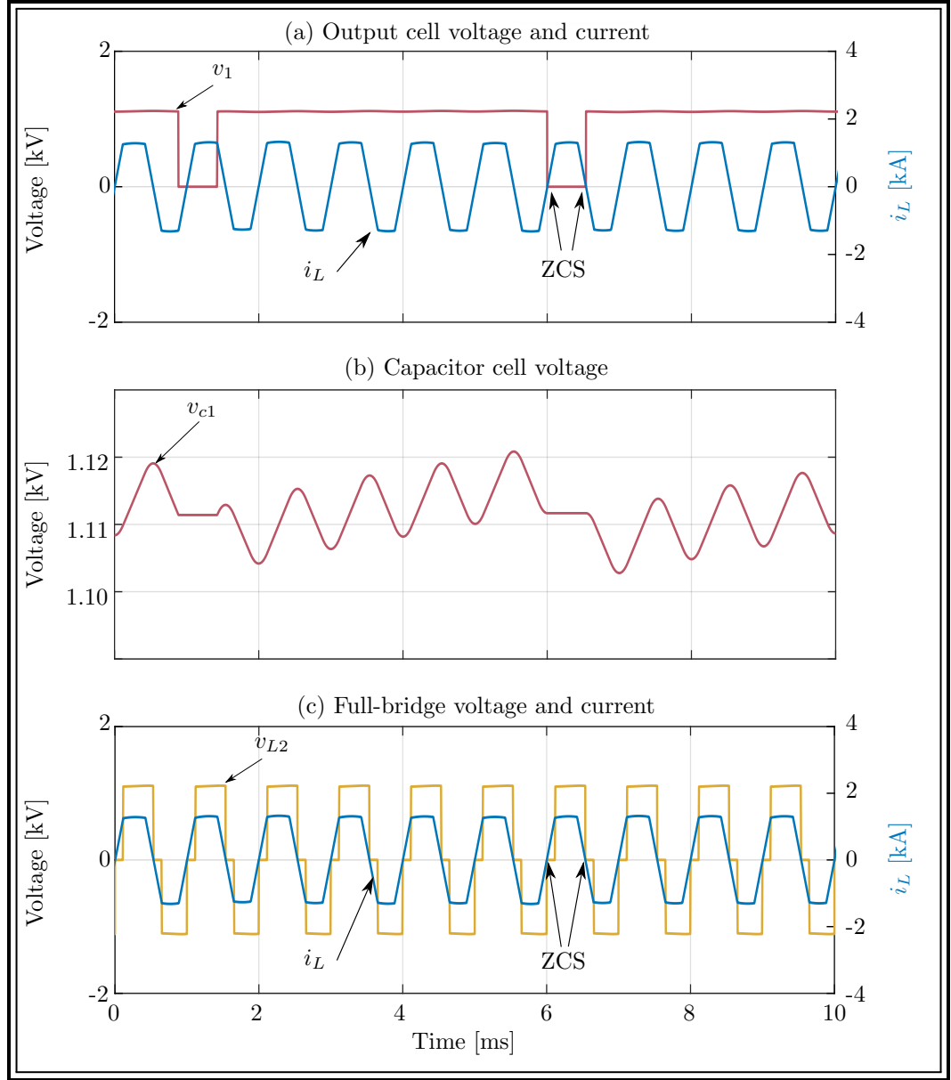
Figure 5.2: Simulation results at full-scale, typical waveforms: (a) Output cell voltage and current, (b) Zoomed capacitor cell voltage, and (c) Output full-bridge voltage and current.
