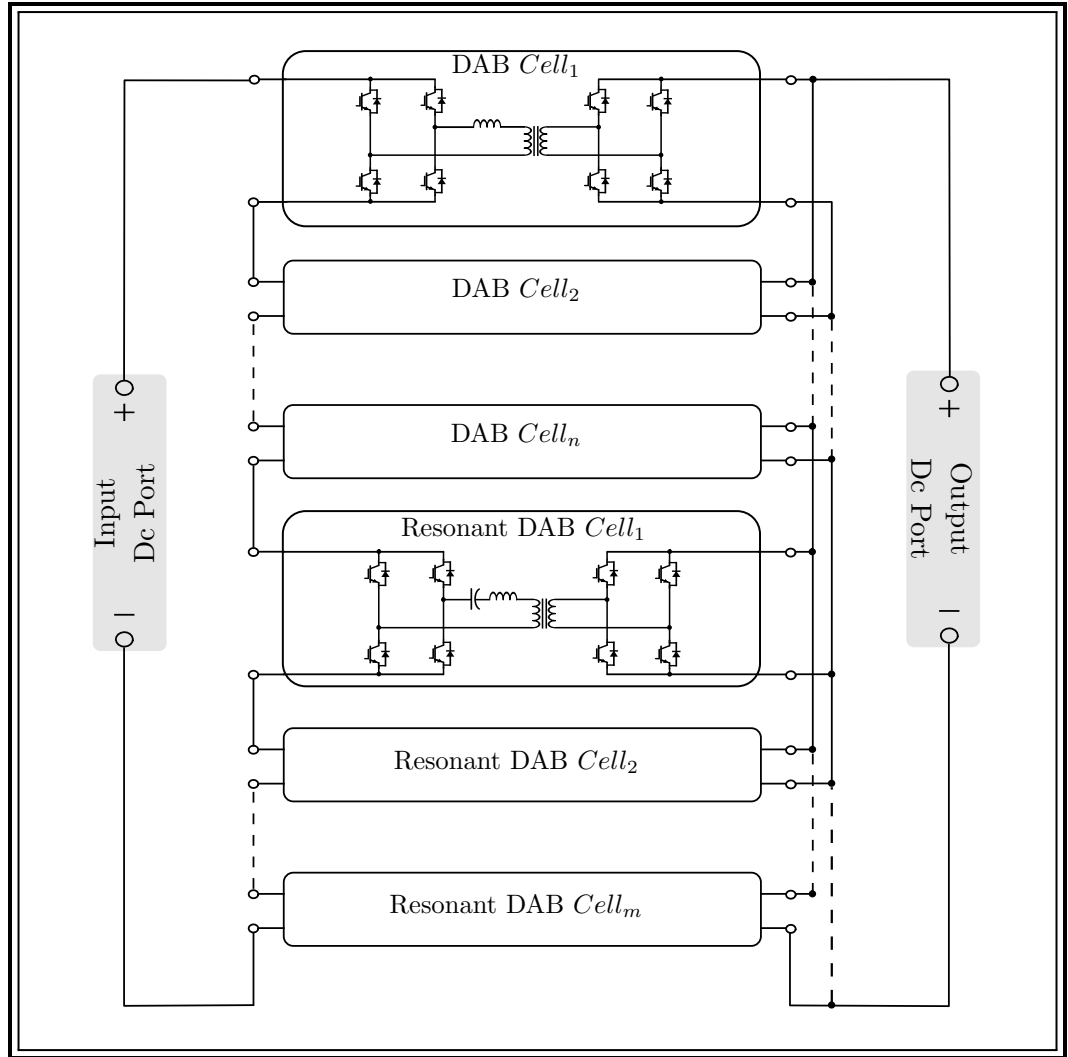
Figure 2.13: Hybrid Multi-DAB converter.
