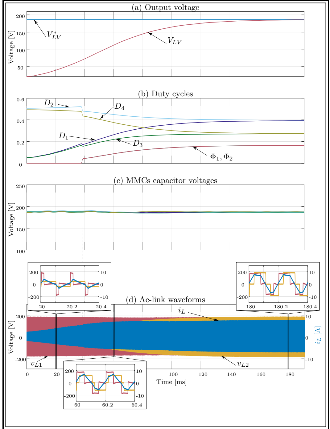
Figure 7.6: Experimental results for V_{LV} step response: (a) Output voltage, (b) Duty cycles, (c) MMC capacitor voltages, and (d) Ac-link waveforms.
