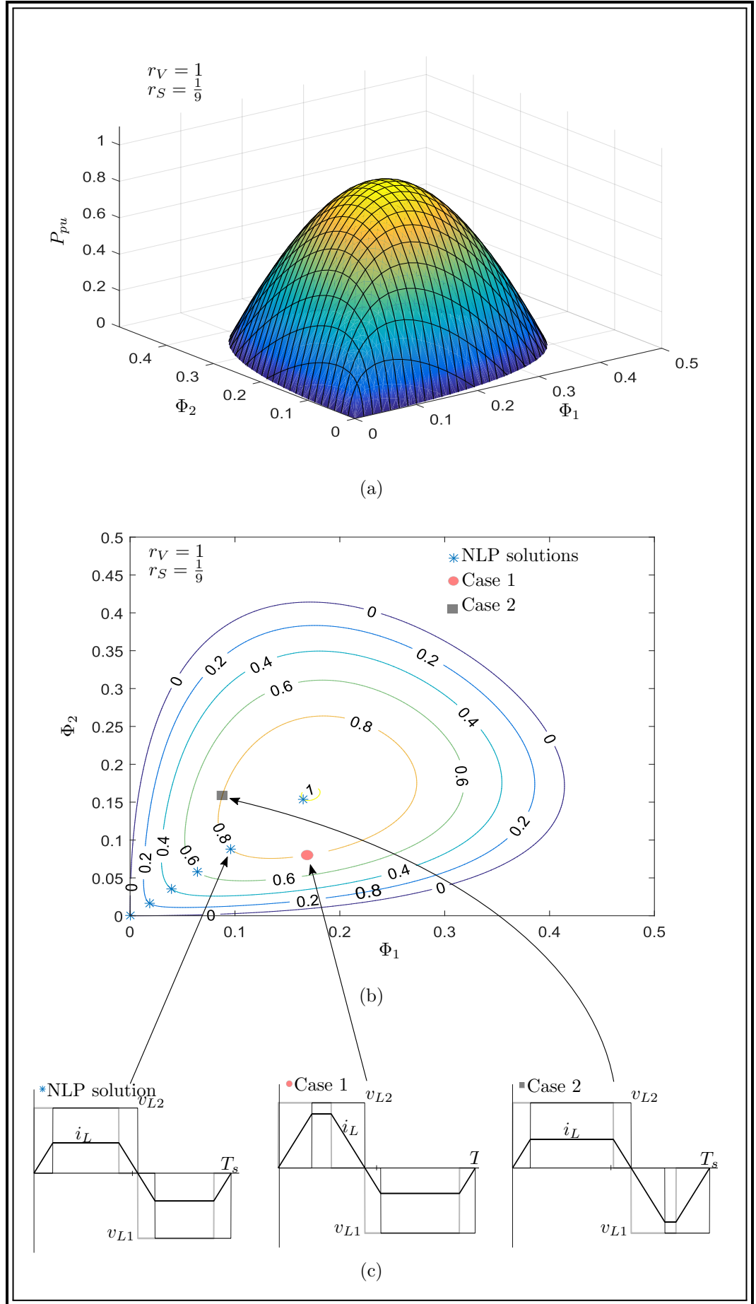
Figure 3.12: Power curves with r_V = 1 and r_S = \frac{1}{9} : (a) Power function, (b) Power contour lines, and (c) Waveforms of feasible solutions for P^* = 0.8 .
