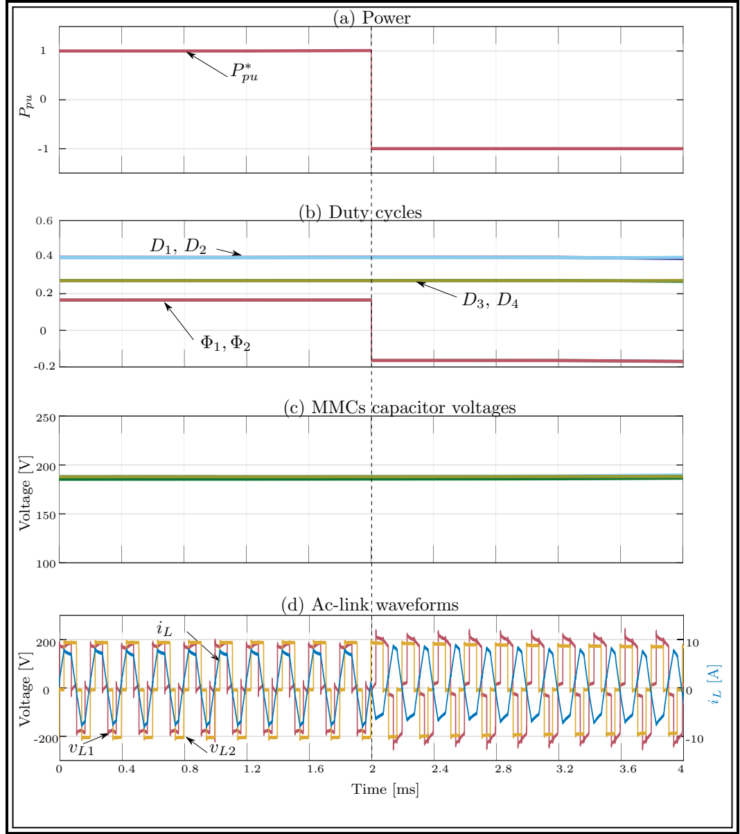
Figure 7.10: Experimental results for maximum power reversal with sorting modulation: (a) Power reference, (b) Duty cycles, (c) MMC capacitor voltages, and (d) Ac-link waveforms.
