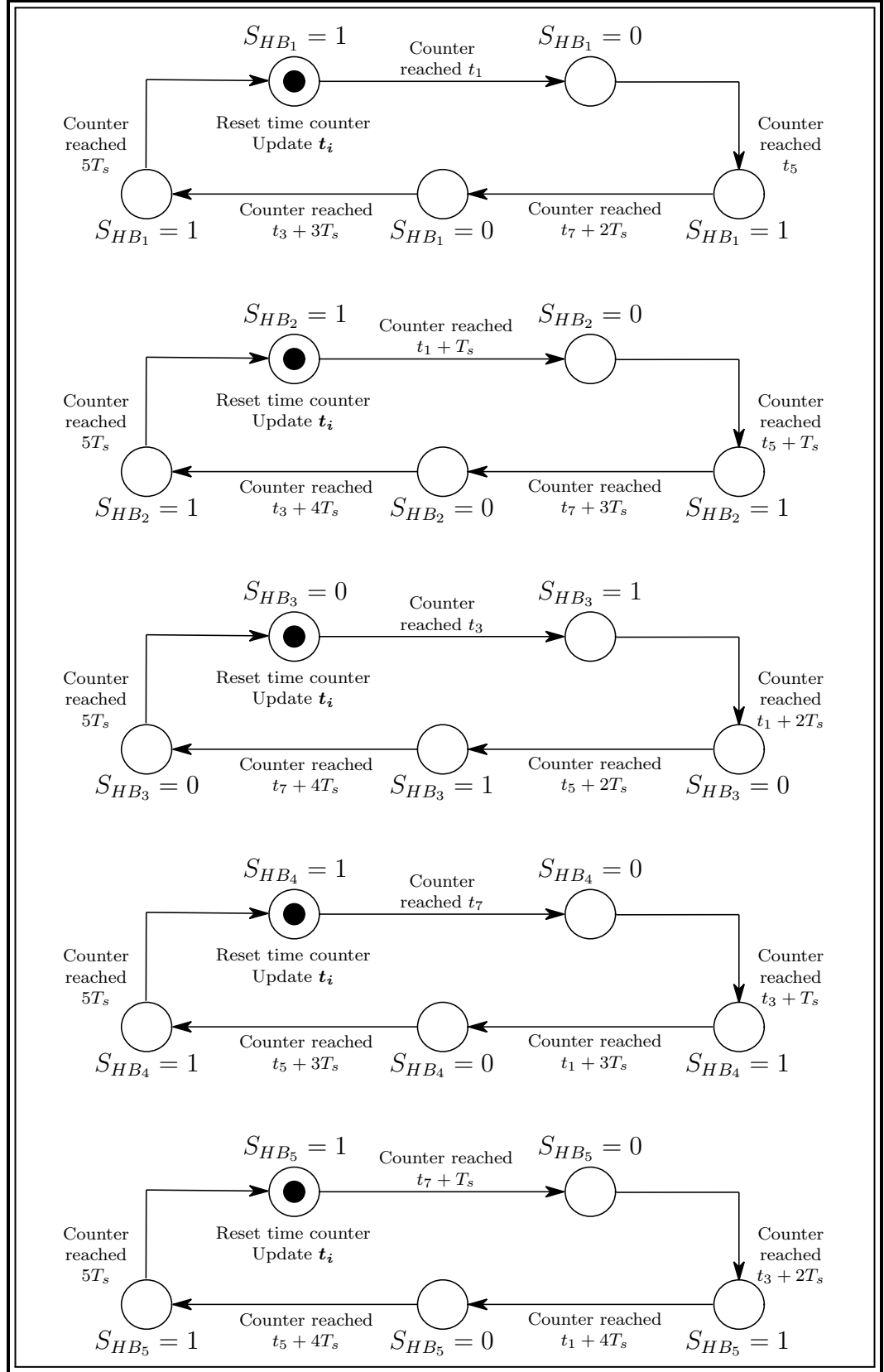
Figure C.1: Half-bridge finite state machines (FSMs) for the case of five cells in the stack and time-controlled phase-shift modulation with j = 2 .
