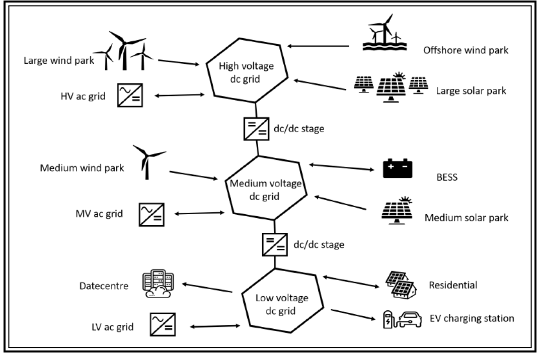
Figure 1.1: Dc grids of different voltage levels.
