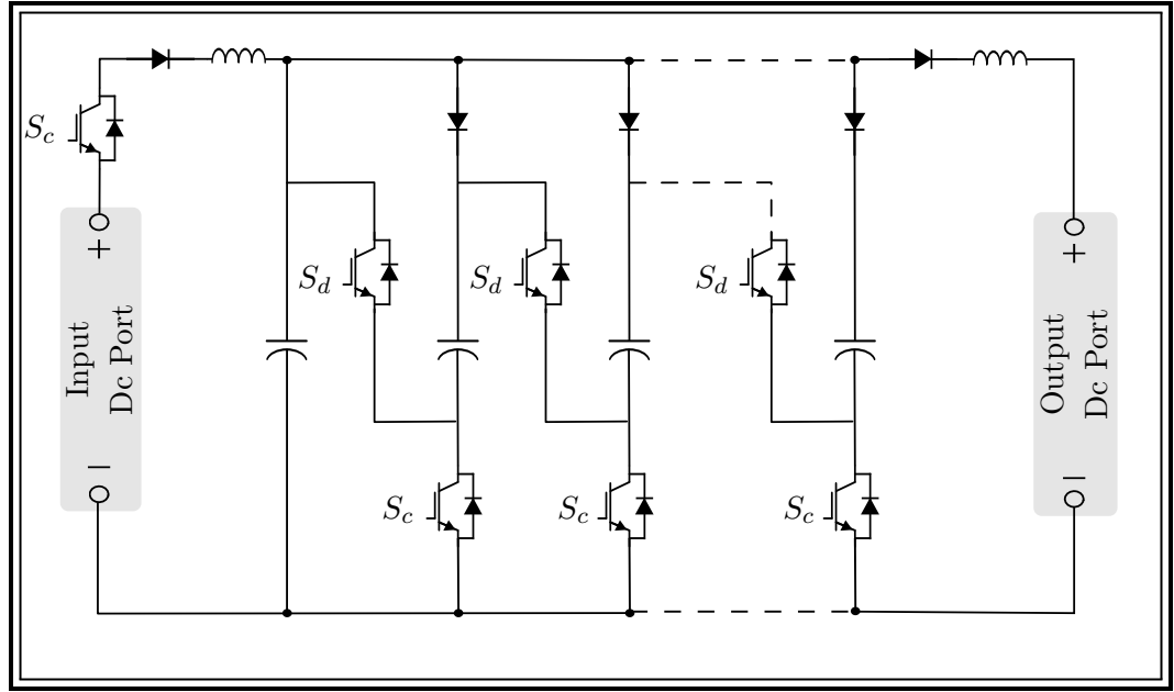
Figure 2.20: Multi-stage resonant converter.
