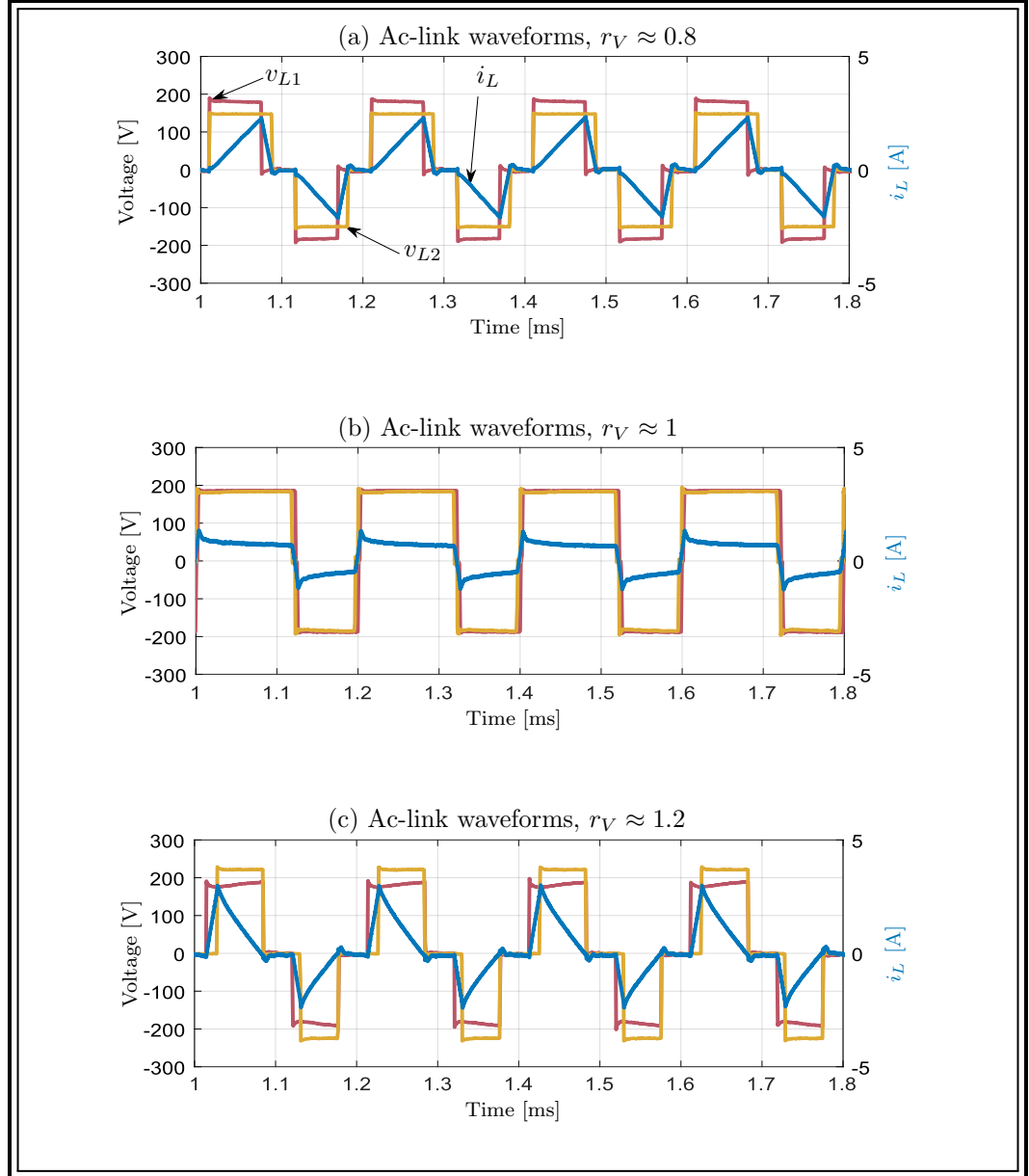
Figure 7.2: Experimental results at steady-state, positive power-flow and low power ( P_{pu} = 0.2 ): (a) Output voltage V_{LV} = 150V ( r_V \approx 0.8 ), (b) Output voltage V_{LV} = 187.5V ( r_V \approx 1 ) and (c) Output voltage V_{LV} = 225V ( r_V \approx 1.2 ).
