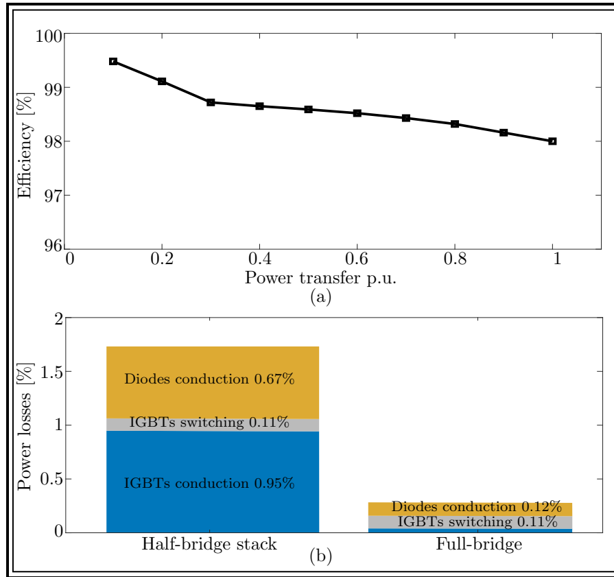
Figure 5.3: Efficiency of simulated converter with r_V = 1 . (a) Efficiency curve vs power transfer, and (b) Power losses distribution at full power.
