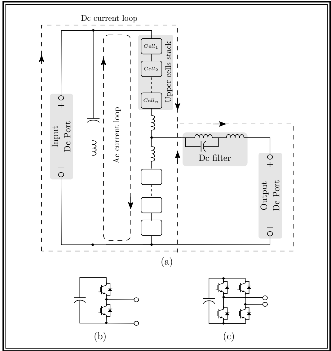
Figure 2.14: Single-leg Buck-Boost structure : (a) Converter topology (b) Half-Bridge cell , and (c) Full-Bridge cell.
