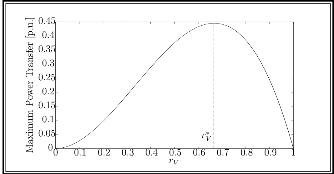
Figure 3.9: Power range limit of P_{\Delta r_V < 1} with r_S = \frac{1}{9} .
