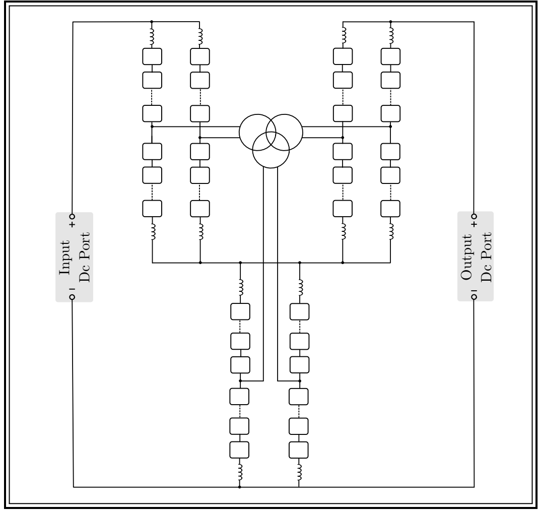
Figure 2.18: Double Wye structure with transformer.
