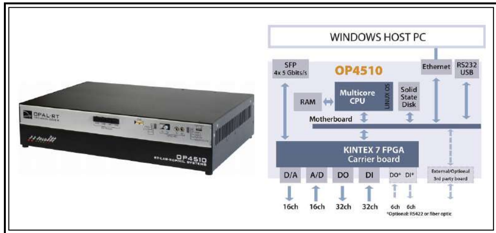
Figure 6.5: Opal-RT 4510 hardware architecture.
