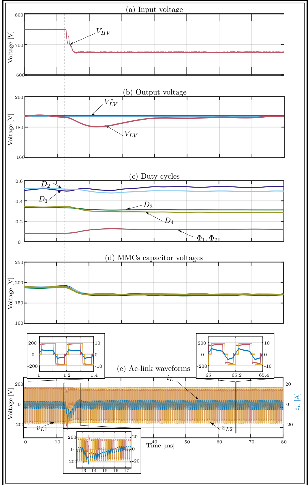
Figure 7.13: Experimental results for V_{HV} step response with sorting modulation: (a) Input voltage, (b) Output voltage, (c) Duty cycles, (d) MMC capacitor voltages, and (e) Ac-link waveforms.
