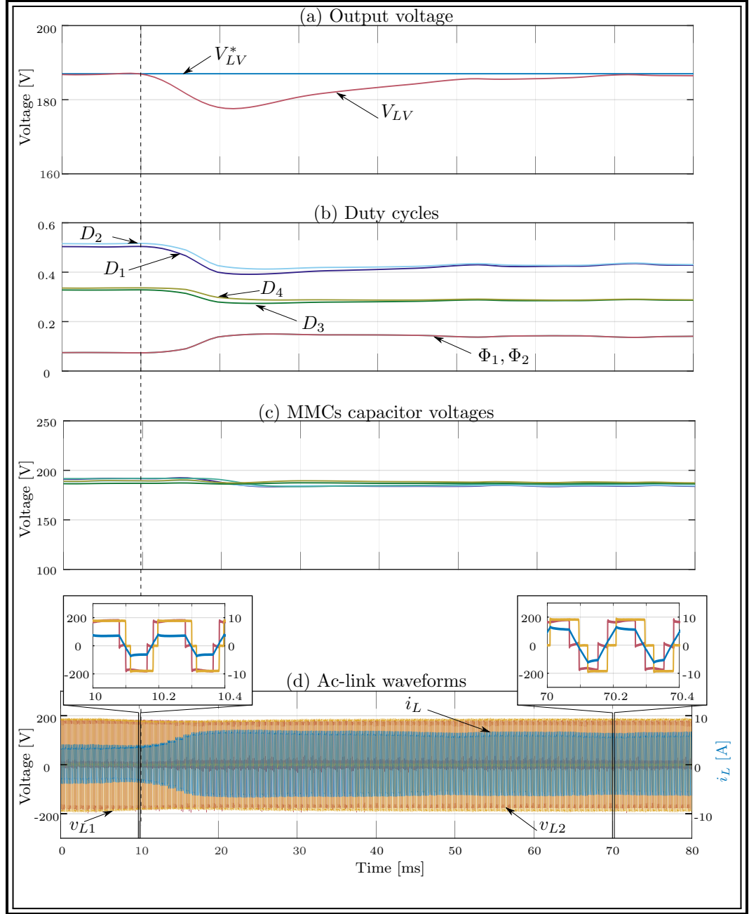
Figure 7.7: Experimental results for R_o step response: (a) Output voltage, (b) Duty cycles, (c) MMC capacitor voltages, and (d) Ac-link waveforms.
