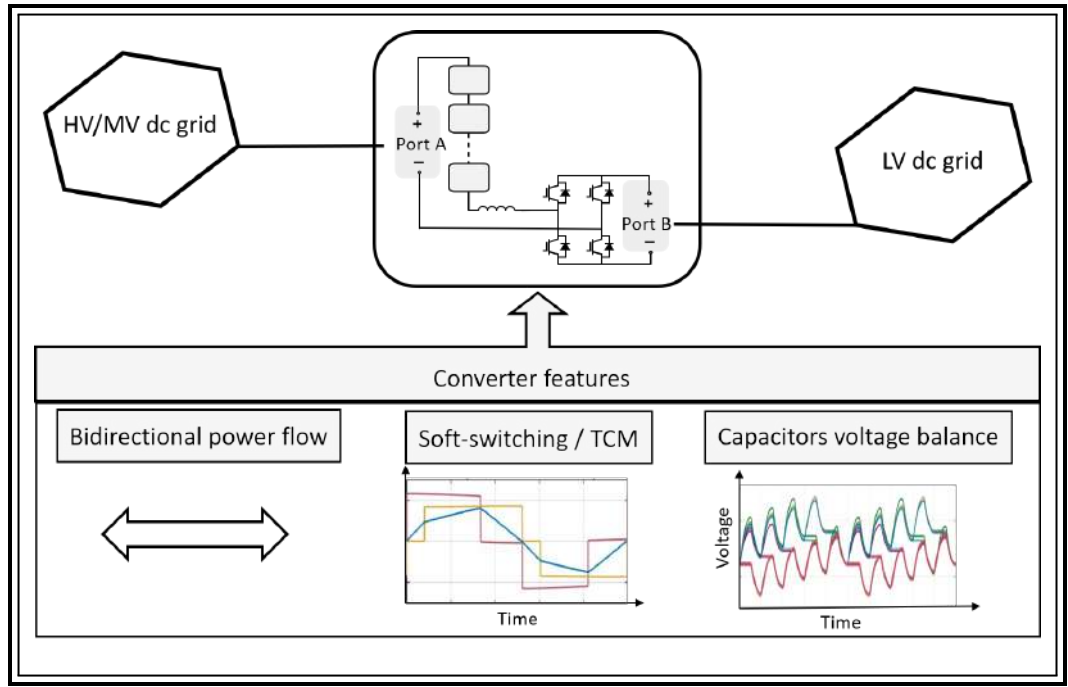
Figure 1.2: High step ratio MMC dc-dc for the interface between dc grids.
