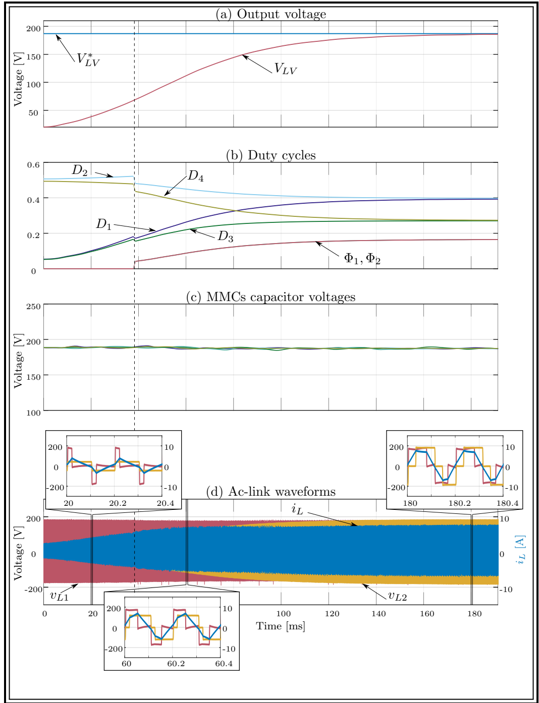
Figure 7.11: Experimental results for V_{LV} step response with sorting modulation: (a) Output voltage, (b) Duty cycles, (c) MMC capacitor voltages, and (d) Ac-link waveforms.
