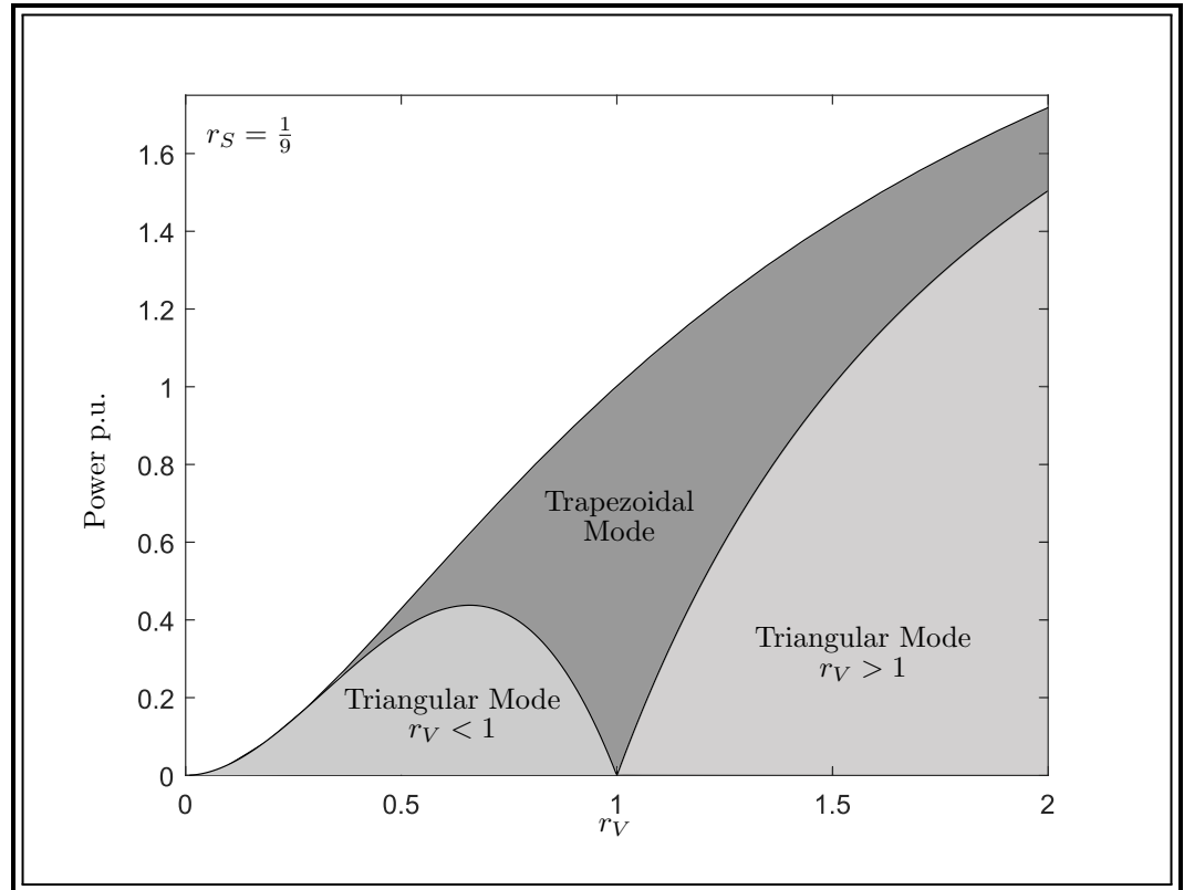
Figure 3.15: Control map for r_S = \frac{1}{9} in the interval r_V = [0, 2] .
