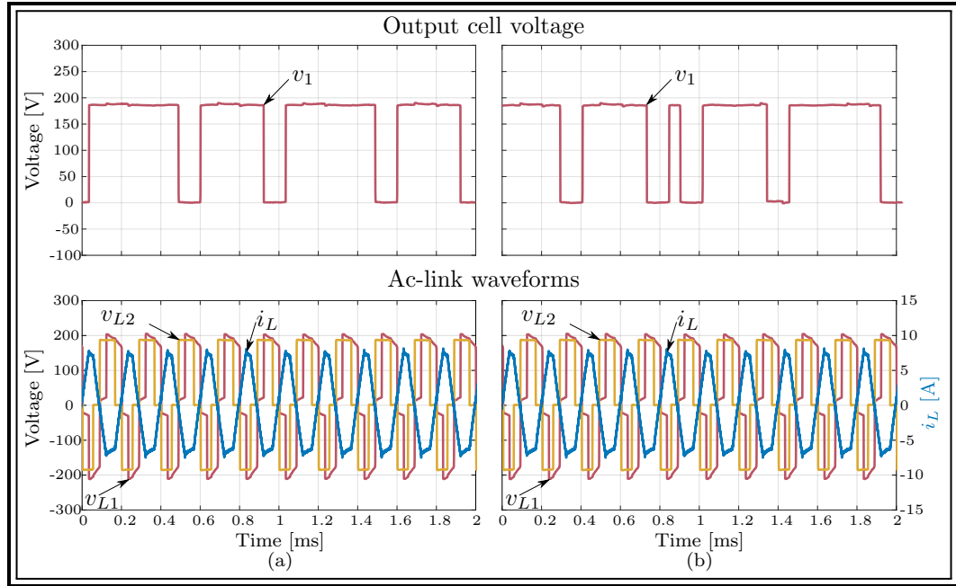
Figure 7.9: Comparative of proposed stack modulation schemes: (a) Phase-shift modulation, (b) Sorting modulation. Steady-state experimental results with r_V = 1 and negative power-flow.
