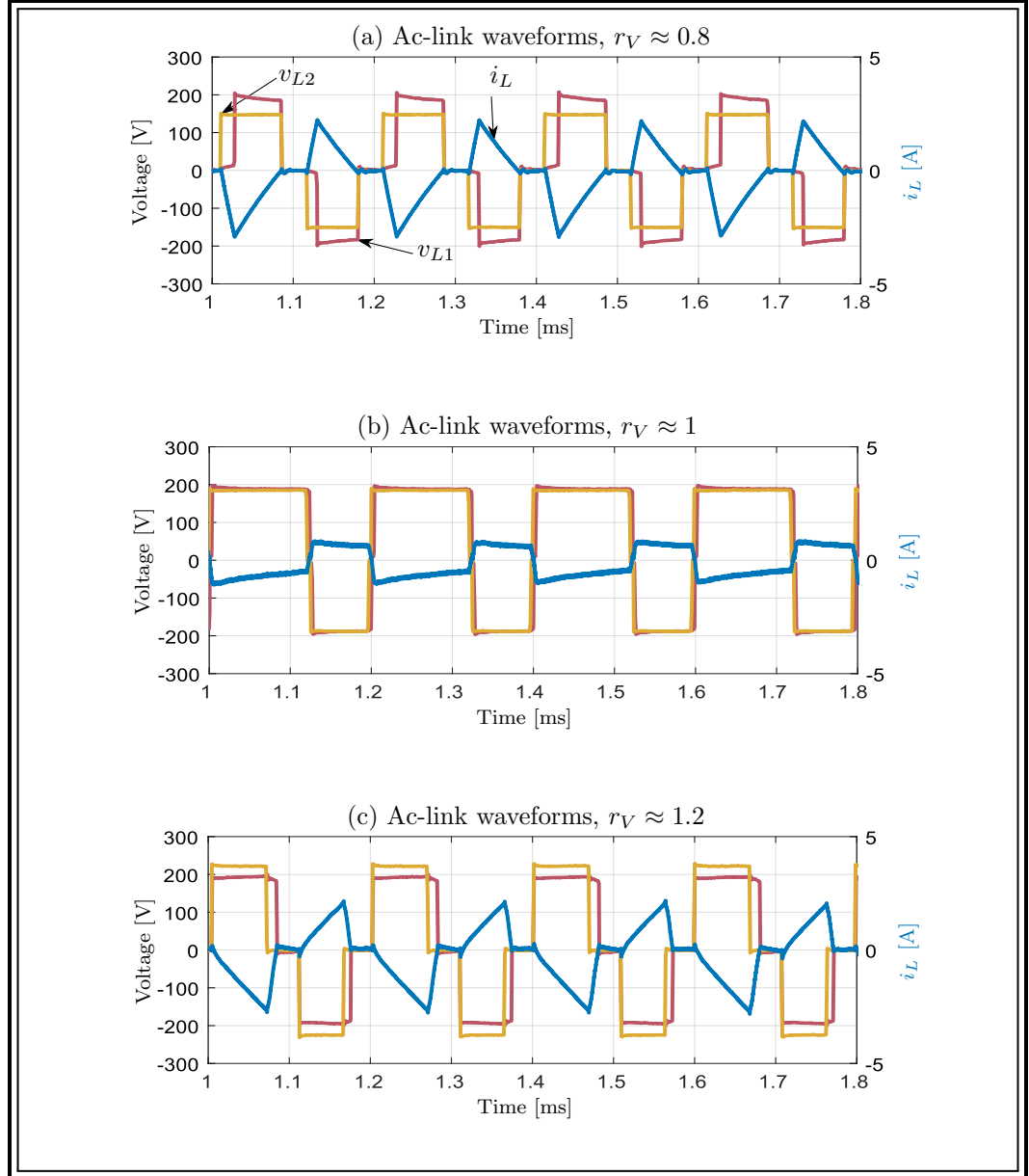
Figure 7.4: Experimental results at steady-state, negative power-flow and low power ( P_{pu} = 0.2 ): (a) Output voltage V_{LV} = 150V ( r_V \approx 0.8 ), (b) Output voltage V_{LV} = 187.5V ( r_V \approx 1 ) and (c) Output voltage V_{LV} = 225V ( r_V \approx 1.2 ).
