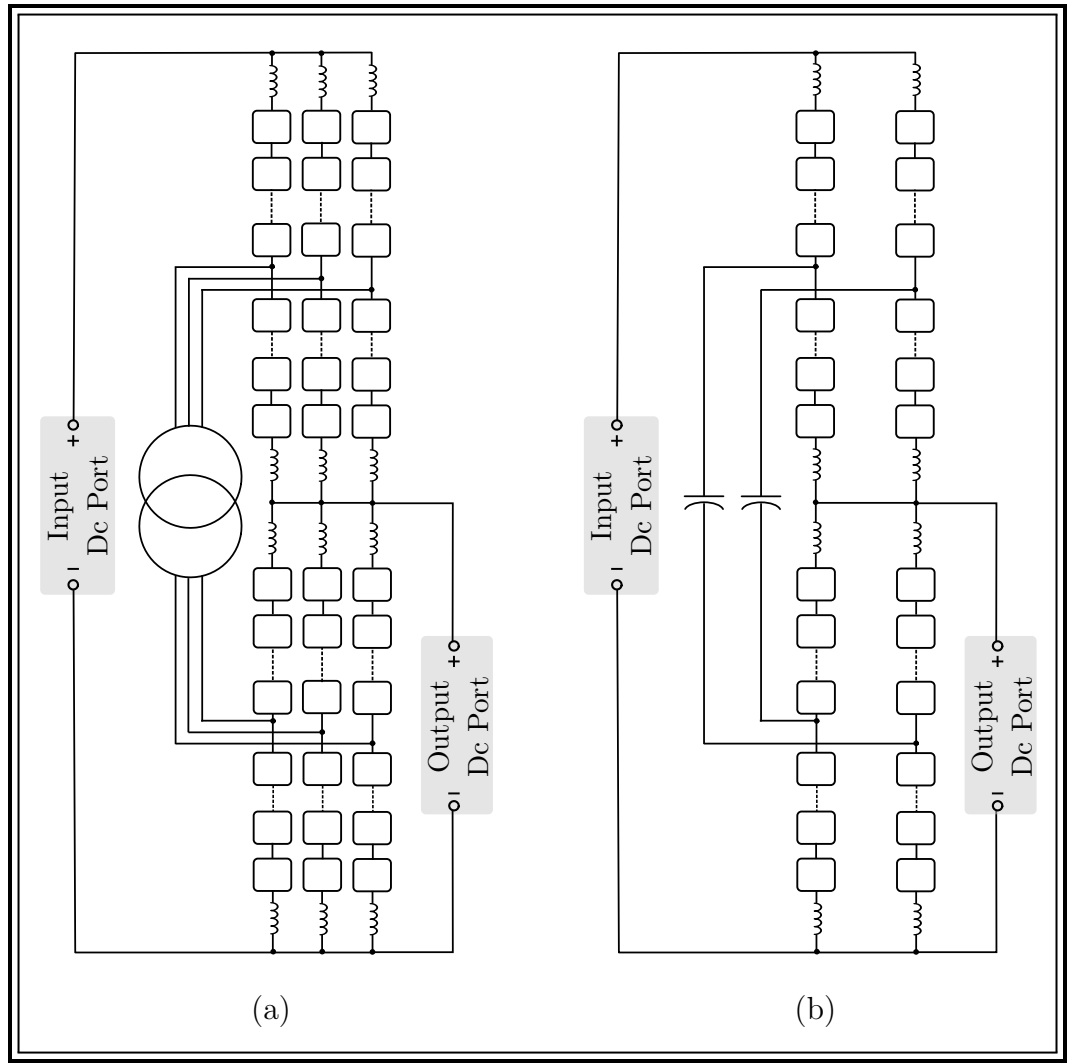
Figure 2.17: Autotransformers structures: (a) 3-Legs DC-Auto, and (b) 2-Legs DC-Auto with capacitors for ac coupling.
