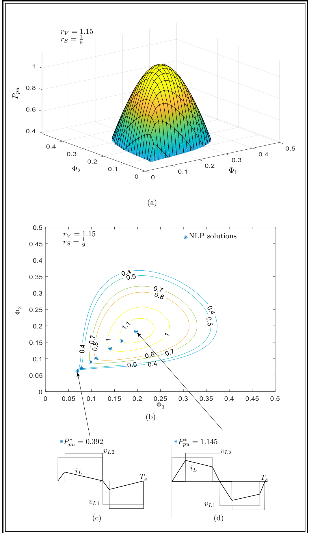
Figure 3.14: Power contour lines with r_V = 1.15 and r_S = \frac{1}{9} : (a) Power function, (b) Power contour lines, and (c)-(d) Waveforms for limit cases using trapezoidal mode.
