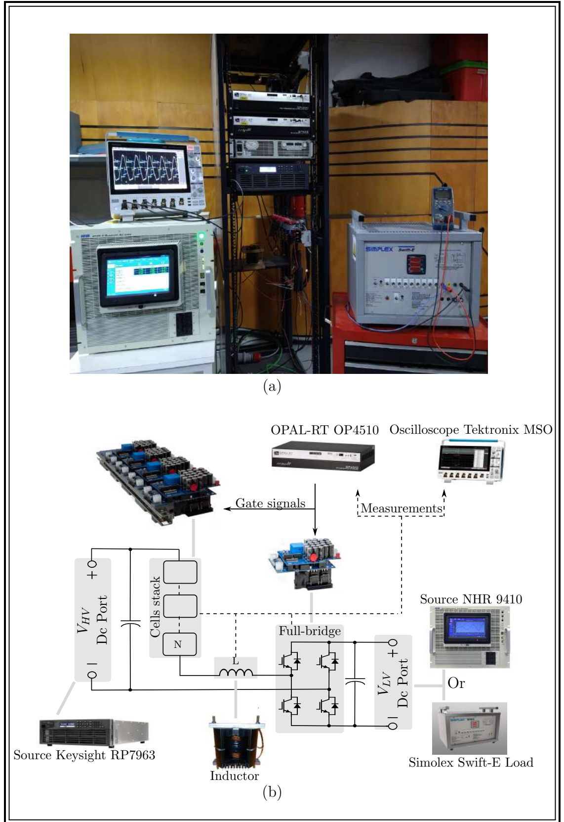
Figure 6.1: Experimental prototype: (a) Lab setup, and (b) Schematic overview.
