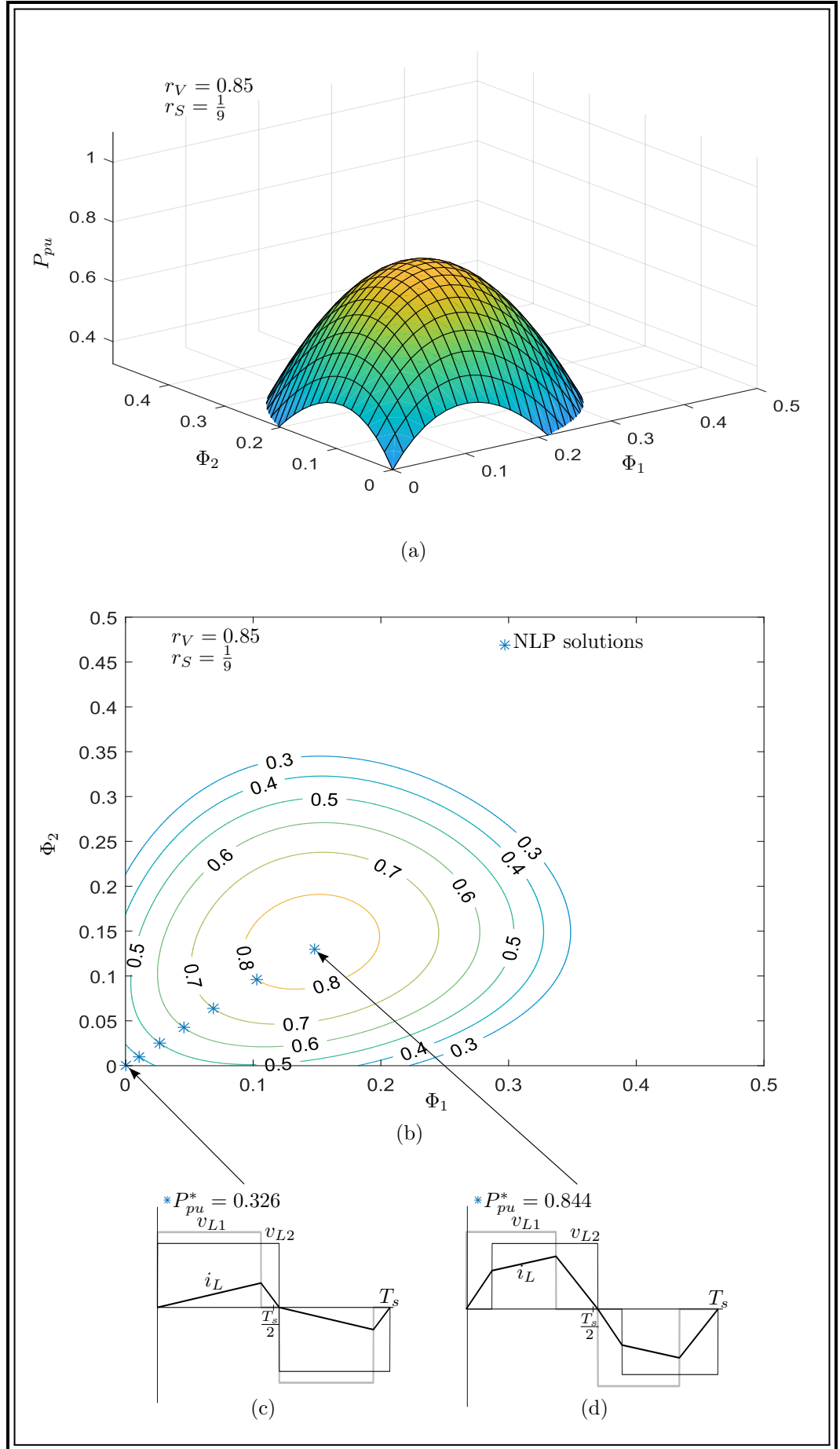
Figure 3.13: Power contour lines with r_V = 0.85 and r_S = \frac{1}{9} : (a) Power function, (b) Power contour lines, and (c)-(d) Waveforms for limit cases using trapezoidal mode.
