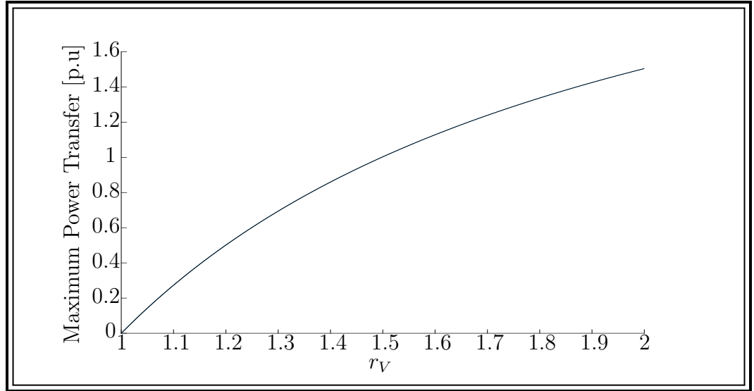
Figure 3.6: Power range of P_{\Delta r_V > 1} with r_S = \frac{1}{9} .
