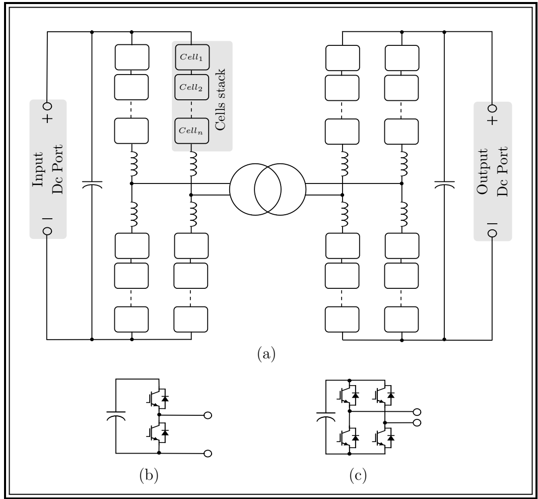
Figure 2.4: (a) FTF-MMC topology, (b) Half-bridge cell, and (c) Full-bridge cell.
