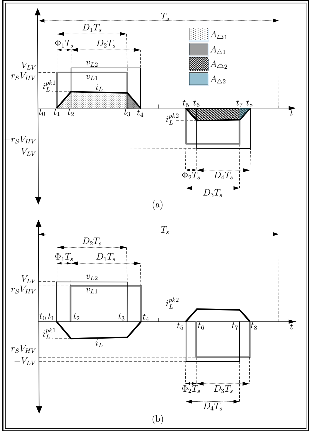
Figure 3.11: Current and voltage waveforms for converter under ZCS trapezoidal modulations: (a) power flow from high-voltage side to low voltage side, and (b) power flow from low-voltage side to high-voltage side.
