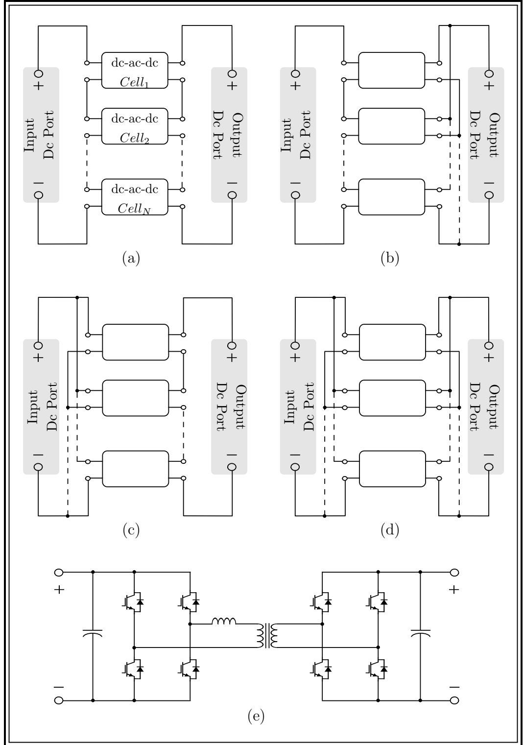
Figure 2.11: Distributed dc-ac-dc converters: (a) ISOS configuration, (b) ISOP configuration, (c) IPOS configuration, (d) IPOP configuration, and (e) DAB cell.
