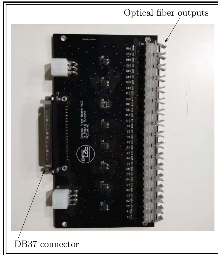
Figure 6.6: Optical fiber PCB.
