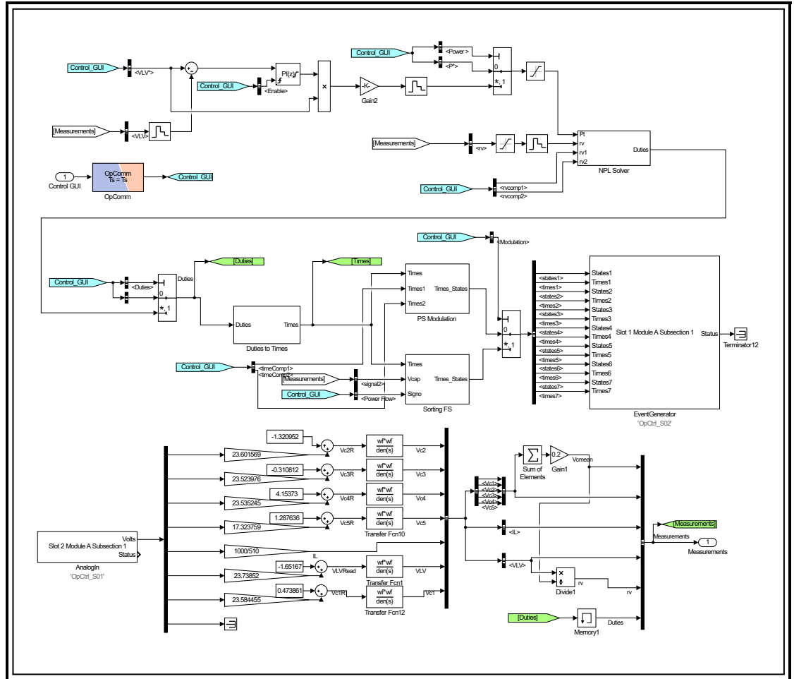
Figure 6.7: Matlab implementation of modulation and control scheme.
