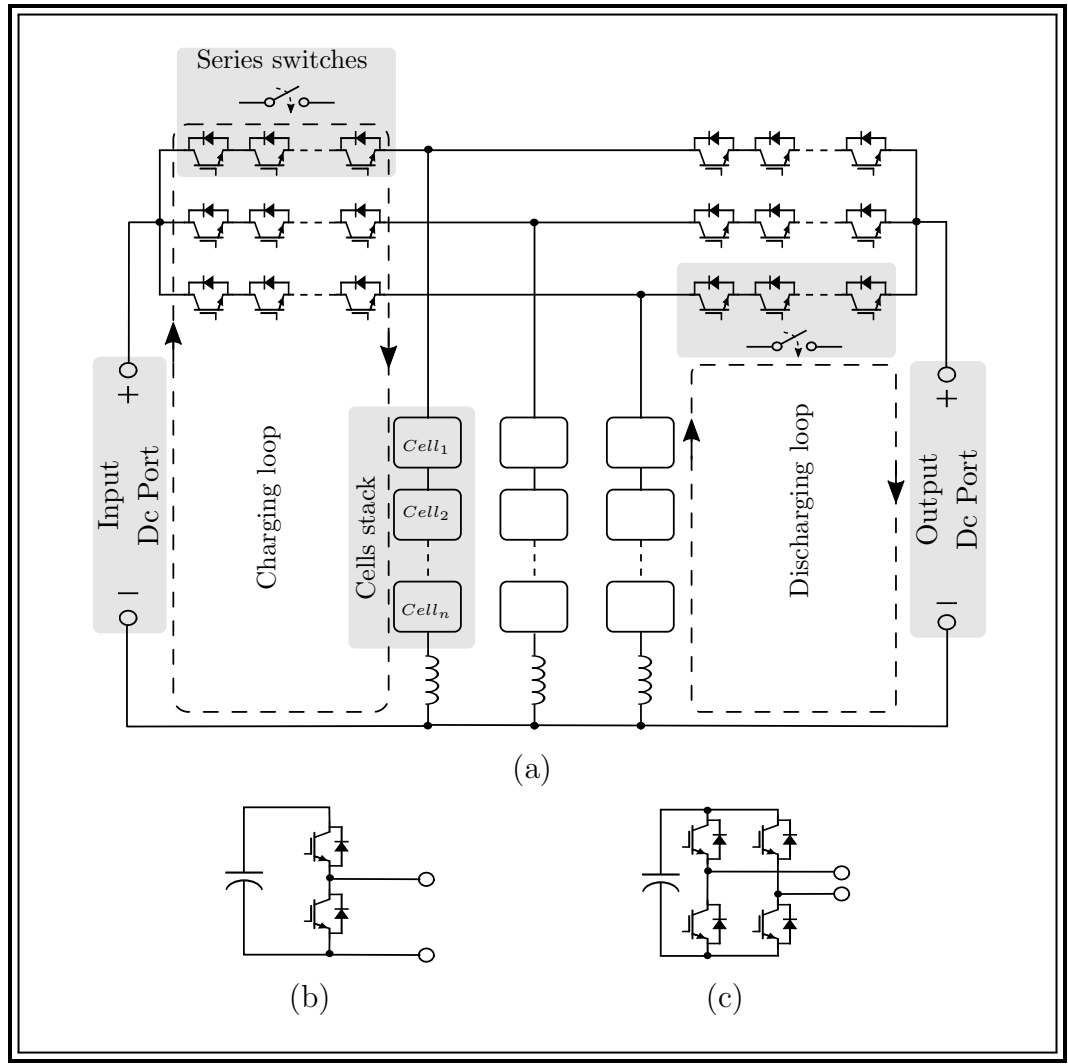
Figure 2.19: Energy accumulator using 3-leg T structure: (a) Topology, (b) Half-bridge cell, and (c) Full-bridge cell.
