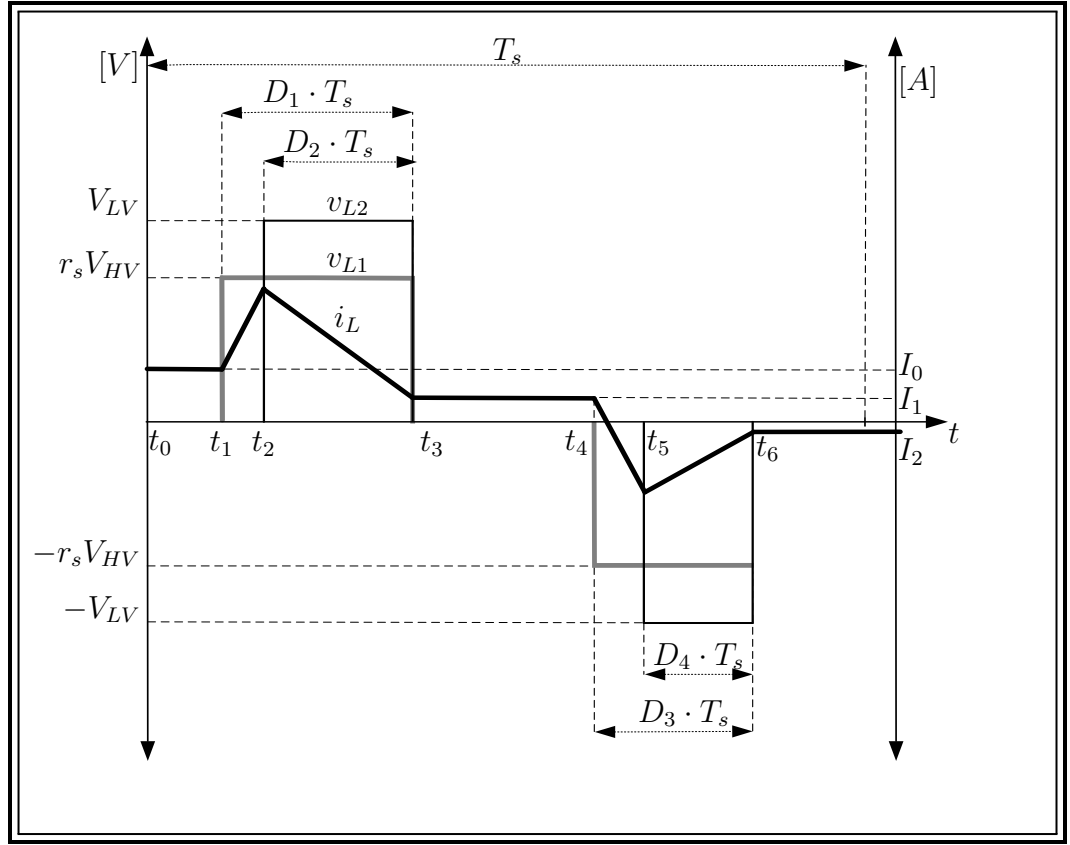
Figure 3.4: General ac-link waveforms for positive power-flow under asymmetrical triangular current mode and r_V > 1 .
