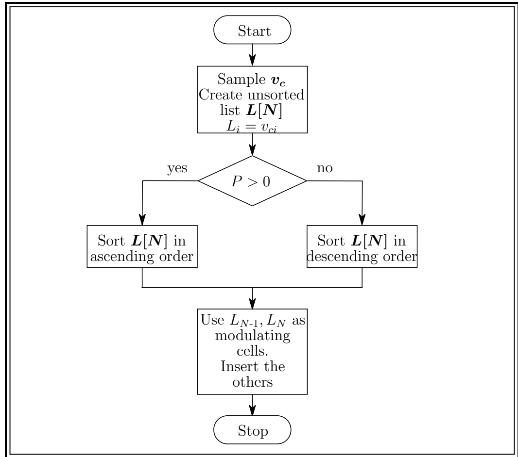
Figure 4.5: Sorting algorithm.
