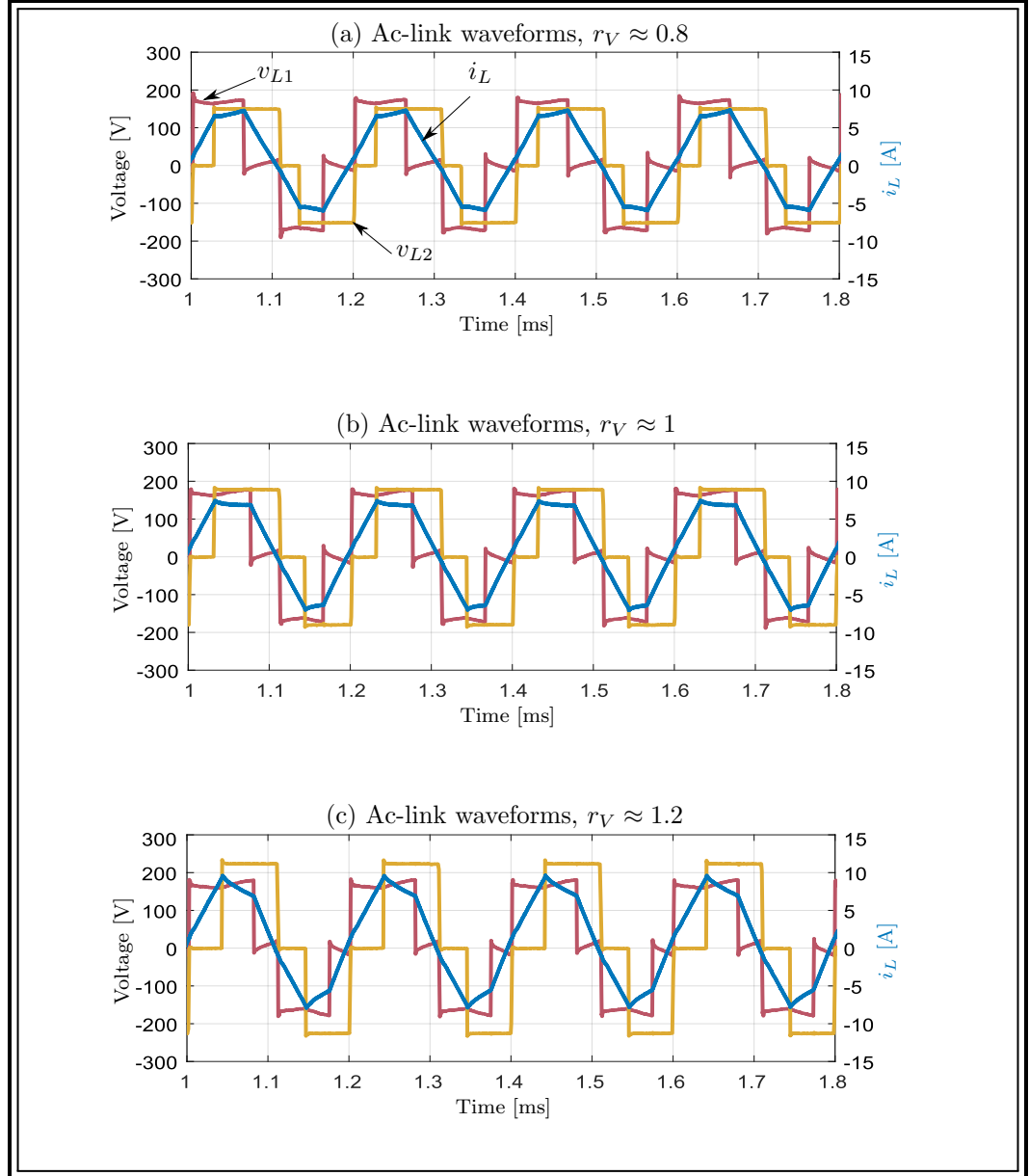
Figure 7.1: Experimental results at steady-state, positive power-flow and maximum power: (a) Output voltage V_{LV} = 150V ( r_V \approx 0.8 ), (b) Output voltage V_{LV} = 187.5V ( r_V \approx 1 ), and (c) Output voltage V_{LV} = 225V ( r_V \approx 1.2 ).
