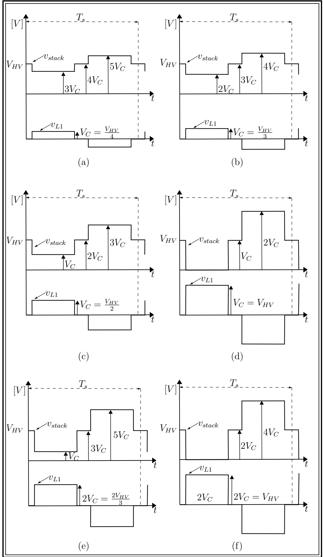
Figure 3.3: Possible switching patterns for a stack formed by five half-bridge cells. (a) choice a, (b) choice b, (c) choice c, (d) choice d, (e) choice, and (f) choice f.
