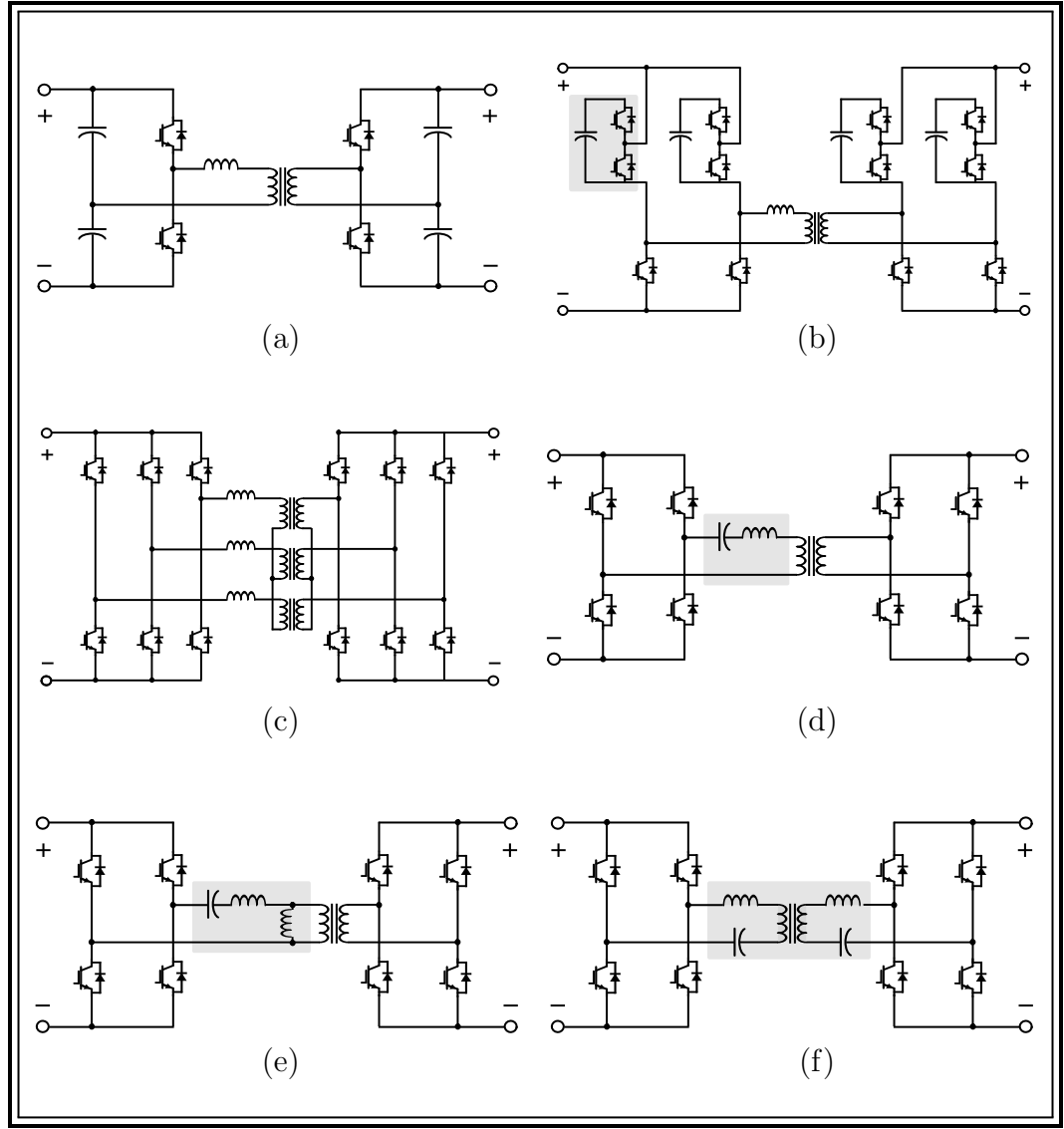
Figure 2.12: Alternatives DAB cells: (a) Dual half-bridge cell, (b) Hybrid-DAB cell, (c) Three-phase DAB cell, (d) LC series resonant DAB cell, (e) LLC resonant DAB, and (f) CLLC resonant DAB.
