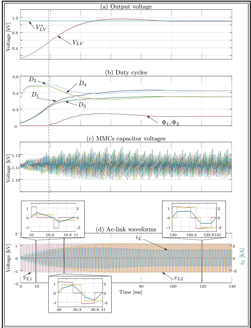
Figure 5.4: Simulation results at full-scale, output voltage step response: (a) Output voltage, (b) Duty cycles, (c) MMC capacitor voltages, and (d) Ac-link inductor waveforms.
