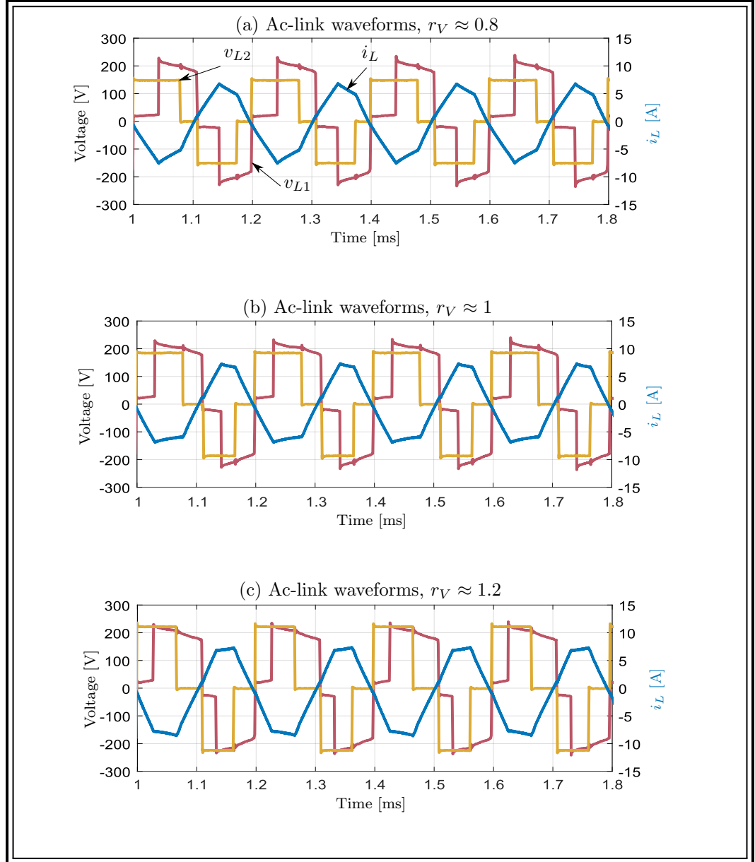
Figure 7.3: Experimental results at steady-state, negative power-flow and maximum power: (a) Output voltage V_{LV} = 150V ( r_V \approx 0.8 ), (b) Output voltage V_{LV} = 187.5V ( r_V \approx 1 ), and (c) Output voltage V_{LV} = 225V ( r_V \approx 1.2 ).
