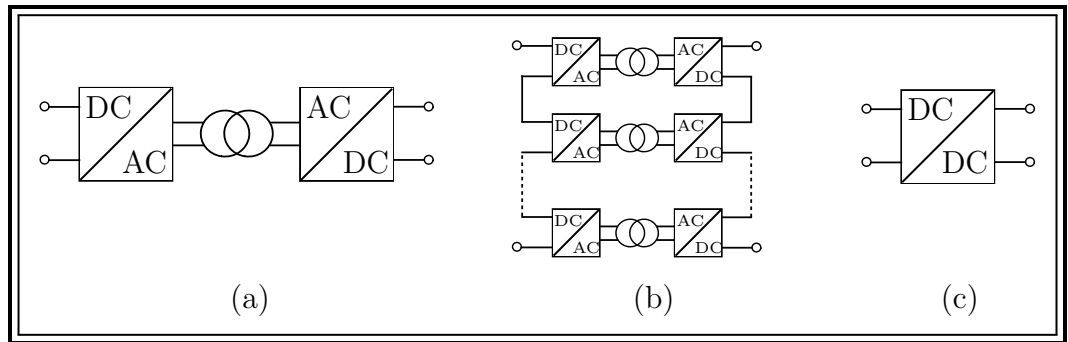
Figure 2.1: Possible structures for dc-dc conversion: (a) Centralised ac-link type , (b) Distributed ac-link type, and (c) Direct dc-dc type.
