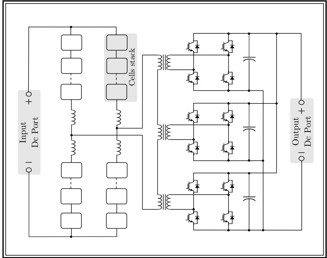
Figure 2.10: Asymmetrical dc-ad-dc MMC with multi-winding transformer.
