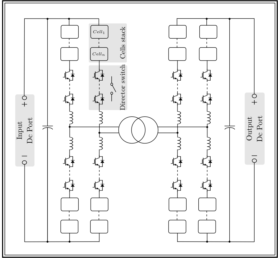
Figure 2.5: Hybrid MMC topology.
