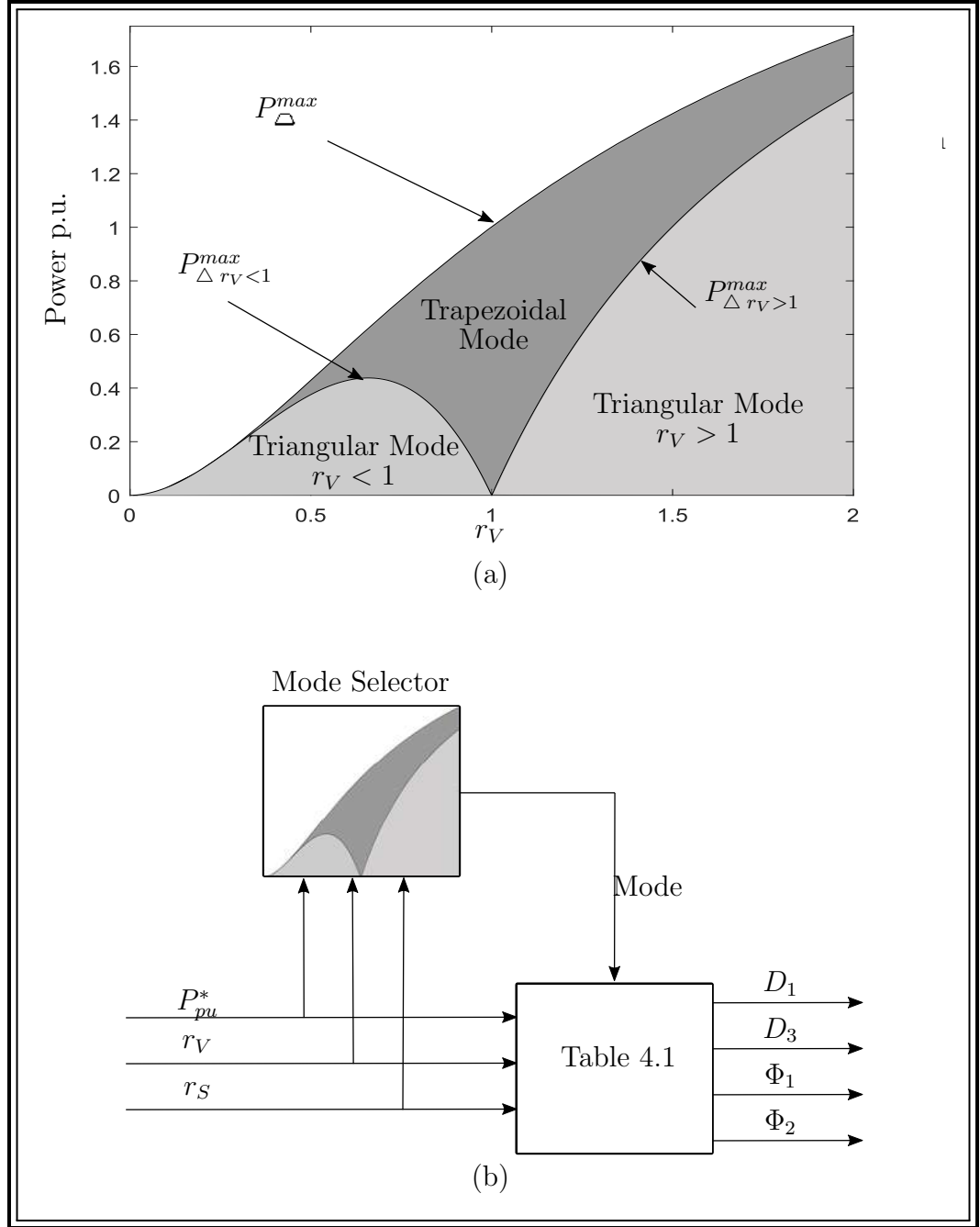
Figure 4.2: Control map implementation: (a) Operating zones, and (b) Control blocks.
