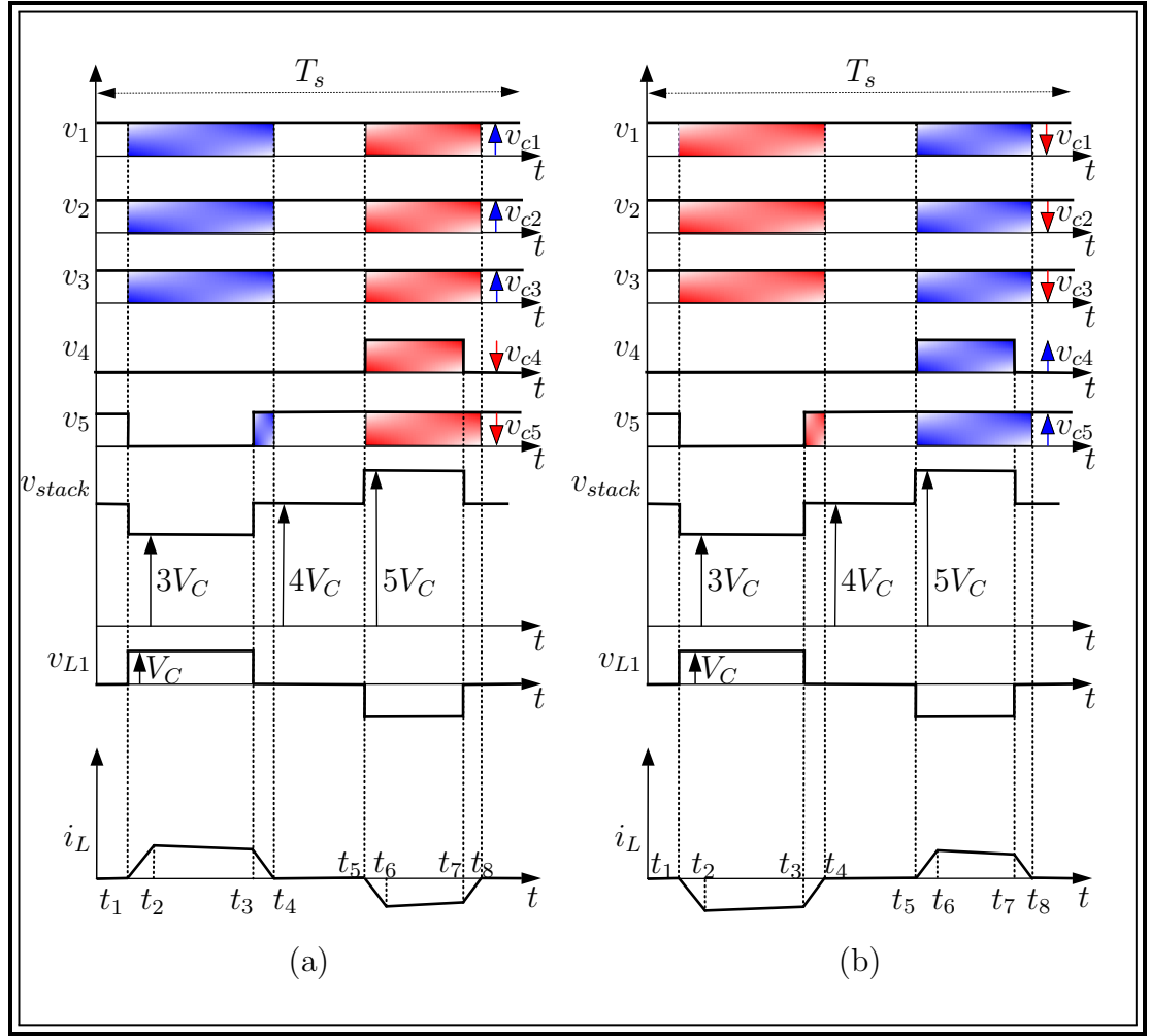
Figure 4.4: Wave-forms in the stack in the period T_s : (a) Positive power-flow, and (b) Negative power-flow.
