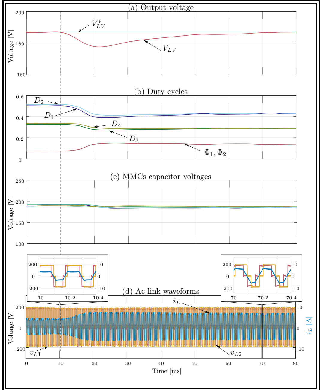
Figure 7.12: Experimental results for R_o step response with sorting modulation: (a) Output voltage, (b) Duty cycles, (c) MMC capacitor voltages, and (d) Ac-link waveforms.
