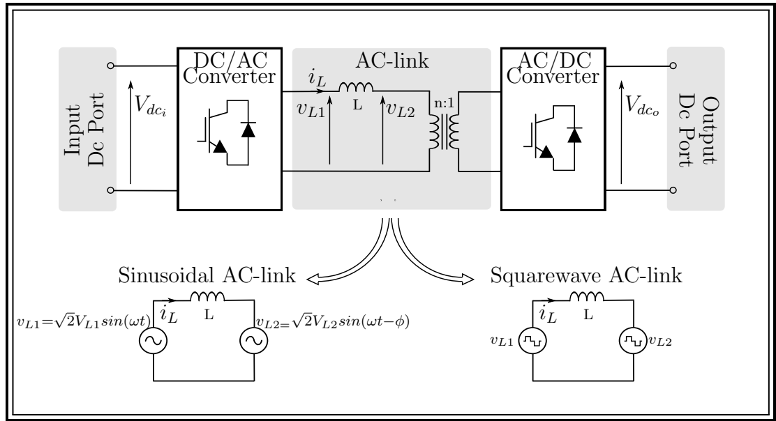
Figure 2.21: General structure of Dc-Dc Converter with AC-link.
