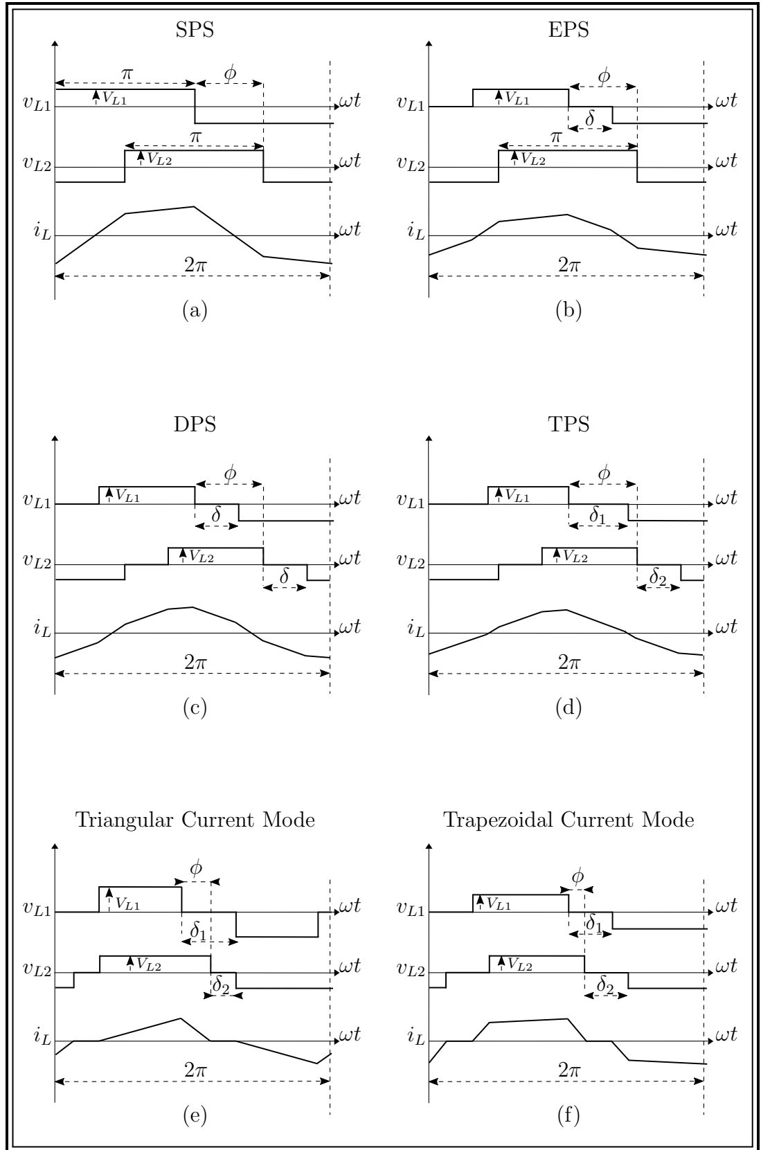
Figure 2.22: Ac link power control strategies: (a) Single phase-shift control (SPS), (b) Extended phase-shift control (EPS), (c) Dual-phase-shift control (DPS), (d) Triple Phase-Shift control (TPS), (e) Triangular Current Mode, and (f) Trapezoidal Current Mode.
