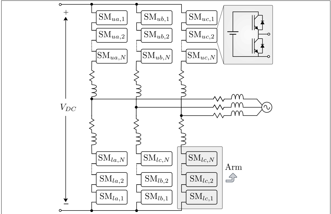
Figure 1.6: MMC-based BESS with BPs directly connected to the SMs.
