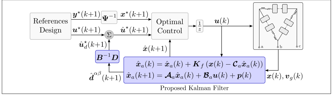
Figure 3.3: Block diagram of the proposed KF observer for steady-state error compensation.
