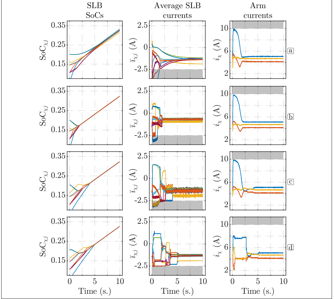
Figure 4.6: Simulation results for different SoC balancing methods. (a) PI-based method [76], (b) sorting-based method [126], (c) MPC strategy [112], and (d) proposed DS-MPC strategy. The shadowed areas represent the imposed safety constraint thresholds.
