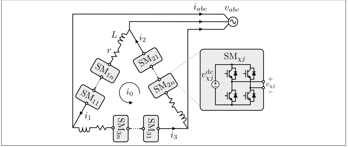
Figure 3.1: Delta-connected CHB converter with n power cells.
