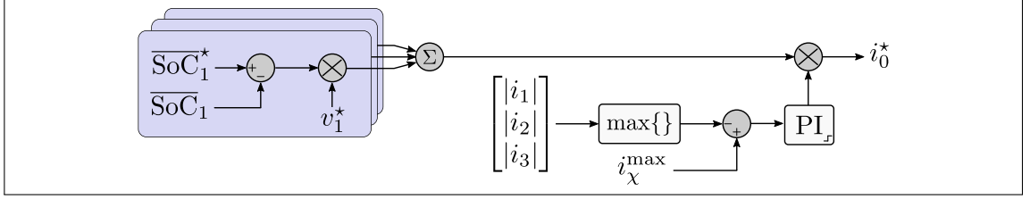
Figure 4.5: Circulating current reference generation scheme applied to the benchmark inter-SM methods analyzed in the simulation results.
