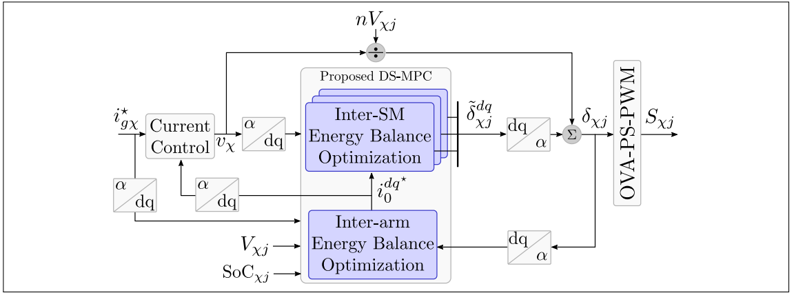
Figure 4.2: Proposed DS-MPC scheme for optimal SoC balancing in \Delta -CHB-BESS.
