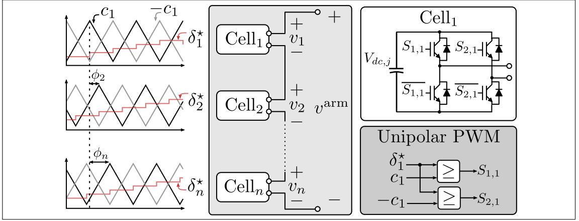
Figure 2.1: CHB converter arm with n SMs using PS-PWM with unipolar modulation.
