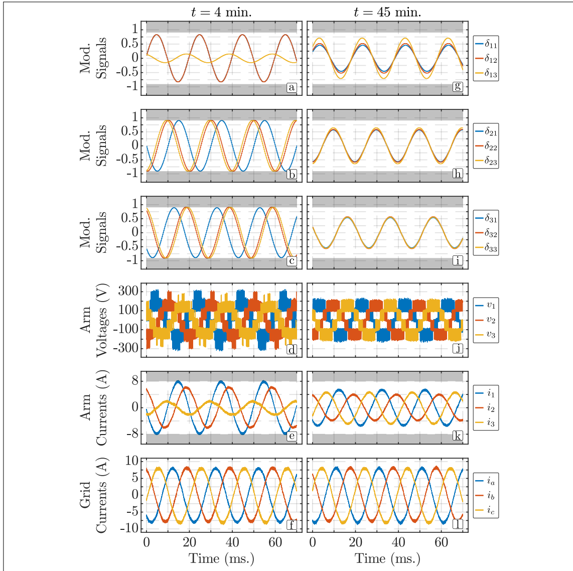
Figure 4.9: Experimental results for the \Delta -CHB waveforms at the beginning and end of the experimental test. The left column shows the converter signals at the beginning of the balancing test. The right column shows the signals close to the end of the test after the SoC balance was achieved.
