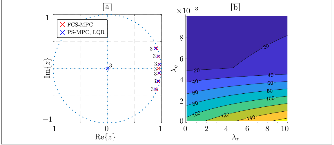
Figure 3.7: KF design. (a) \mathbf{A}_{\text{obs}} eigenvalues in the z -plane, (b) sensitivity analysis for the observer settling time in milliseconds.
