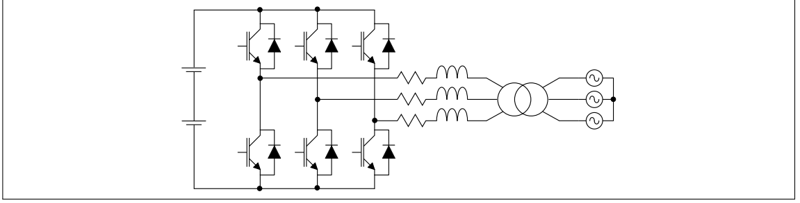
Figure 1.2: BESS based on the conventional 2L-VSC.
