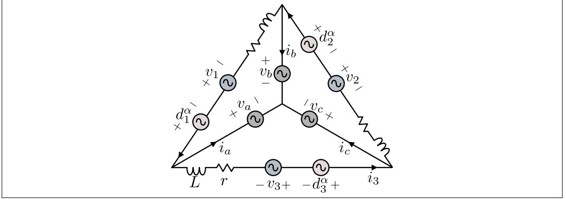
Figure 3.2: Equivalent continuous-time circuit diagram of the augmented state-space model for the CHB converter, where d_{\chi}^{\alpha} = (d_{\chi 1}^{\alpha} + d_{\chi 3}^{\alpha} + d_{\chi 5}^{\alpha}) \frac{r\gamma}{L(\gamma-1)} , \gamma = e^{T_s r/L} .
