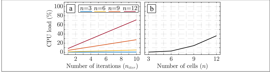
Figure 2.7: Execution time of the proposed OVA-PS-PWM in percentages of the total available time. (a) CPU load for different number of SMs and iterations, (b) CPU load for 8 iterations for different number of SMs.
