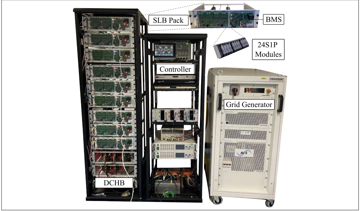
Figure 4.7: \Delta -CHB-BESS experimental prototype with 9 SMs and SLBs.
