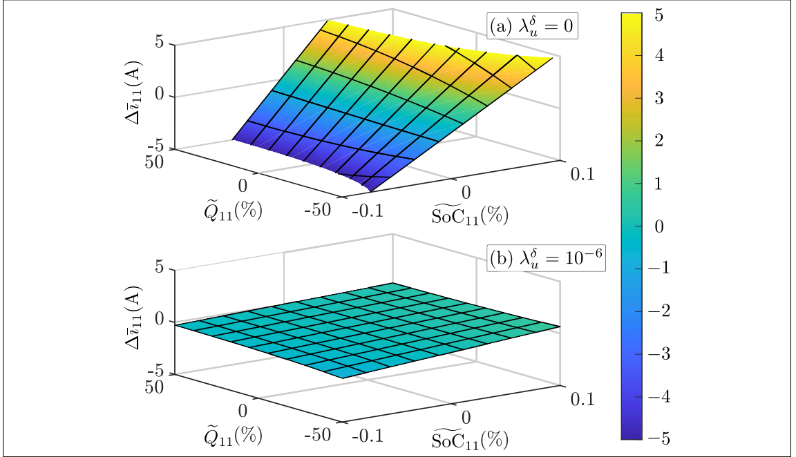
Figure 4.3: Numerical example of the current error at the unconstrained battery current solution due to disturbances in the capacity values and SoC estimates. (a) dead-beat solution, (b) proposed DS-MPC strategy inter-SM solution.
