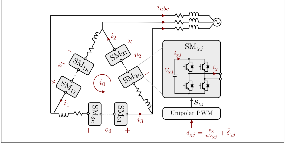
Figure 4.1: Current and voltage definitions for the three-phase \Delta -CHB converter topology with n SMs per arm and batteries directly connected to each SM analyzed in this chapter.
