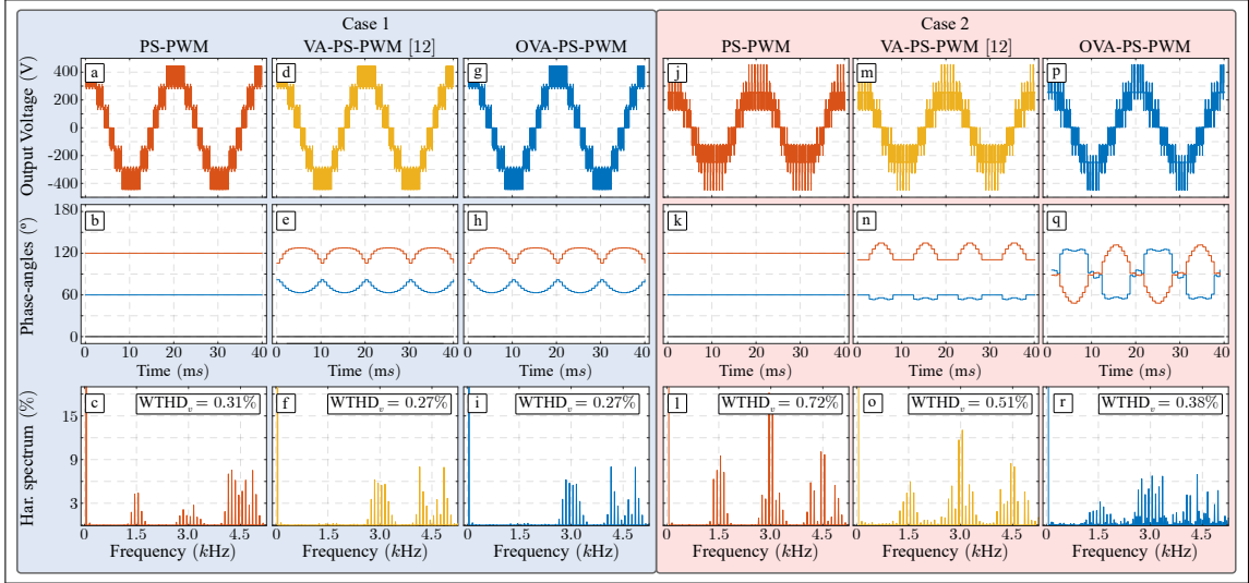
Figure 2.3: CHB output voltage, PS-angles, and voltage harmonic spectra for the simulated cases 1 and 2.
