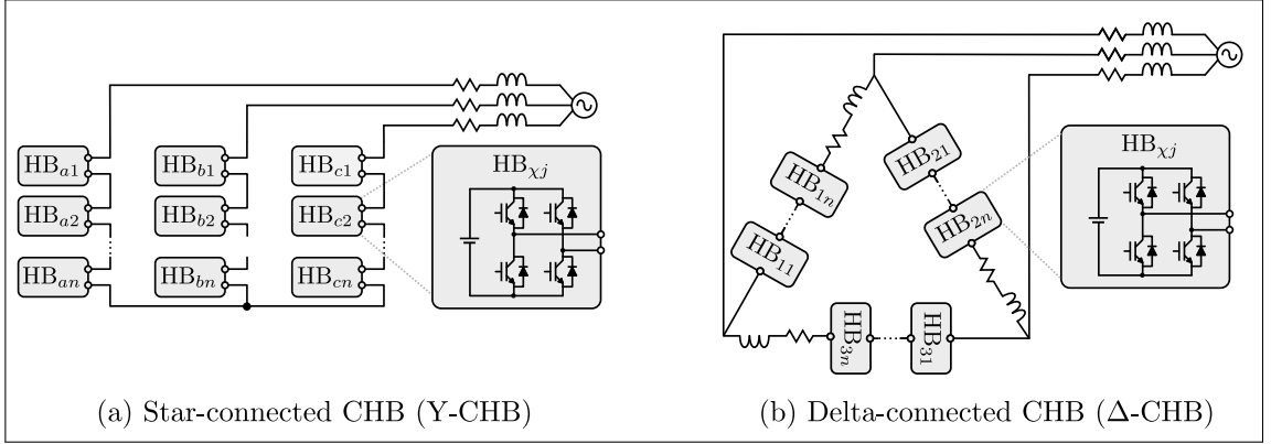
Figure 1.5: CHB converter-based BESS with BPs directly connected to the SMs. (a) star configuration, (b) delta configuration.
