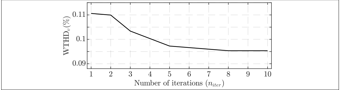
Figure 2.6: Simulation results for the impact of the number of iterations of the OVA-PS-PWM algorithm in the CHB output voltage WTHD.
