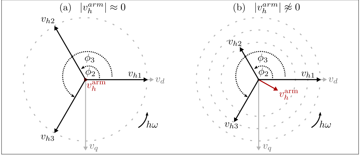
Figure 2.2: Representation of the h -st output voltage harmonic component for a 3-SM CHB converter in the rotating synchronous dq -frame for conventional PS-angles. (a) balanced operation, (b) unbalanced operation.
