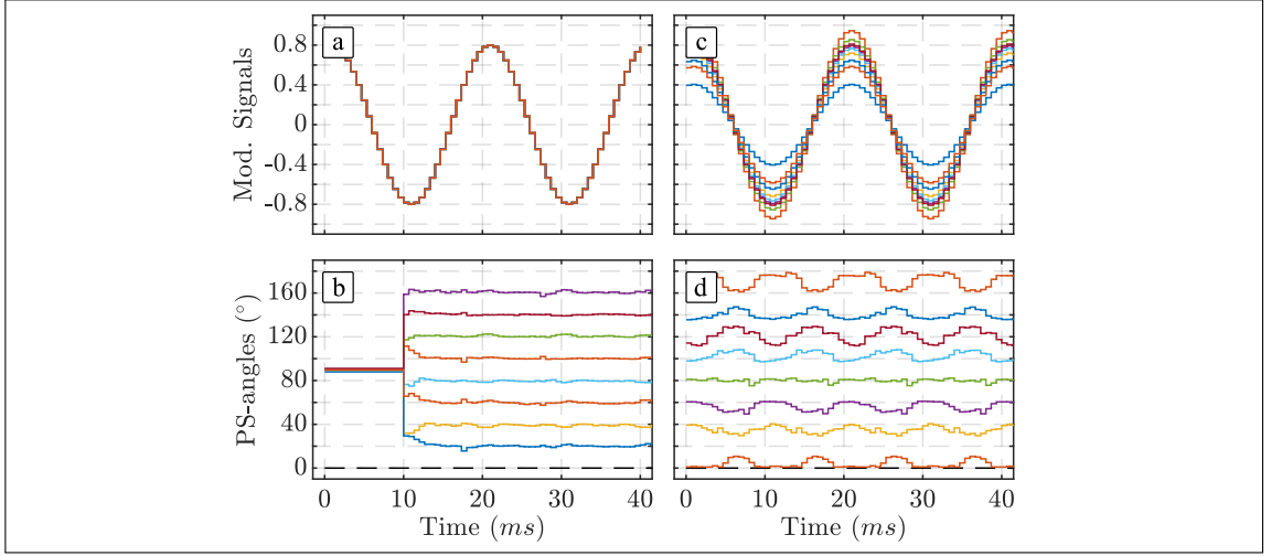
Figure 2.9: PS-angles and modulating signals for the experimental results. (a)-(b) shows the convergence of the proposed OVA-PS-PWM for the balanced case. (c)-(d) shows the steady-state signals for the unbalanced case.
