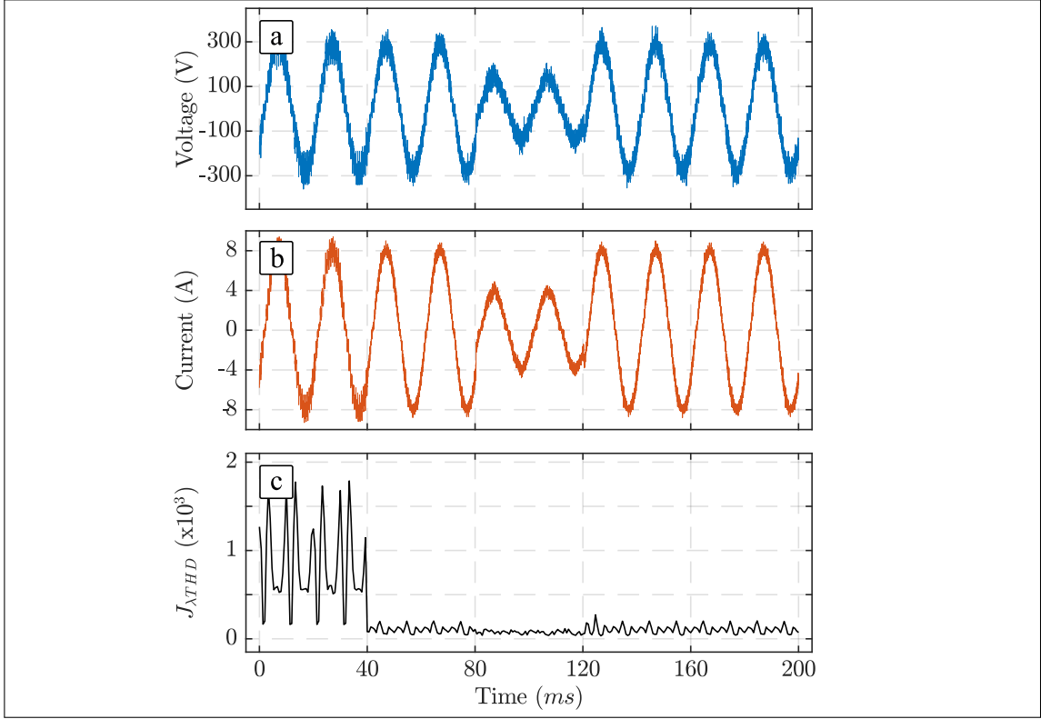
Figure 2.10: Transient response of the proposed OVA-PS-PWM after enabled at 40 ms. (a) CHB output voltage, (b) output current, (c) instantaneous cost function J_{\lambda THD}(k) value.
