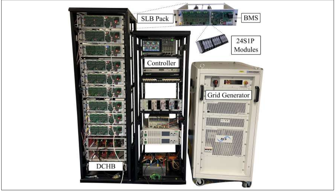
Figure 3.4: Three-phase CHB-BESS converter prototype.
