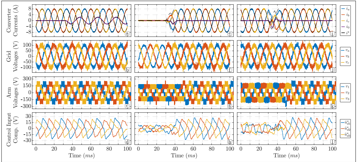
Figure 3.8: Experimental results for the proposed KF strategy under transients for an LQR. (a)-(d) shows a transient response for a circulating current step change, (e)-(h) shows an active power reference change of 1.2 kW, and (j)-(l) shows transient reversing the power flow from -1.2 kW to 1.2 kW.
