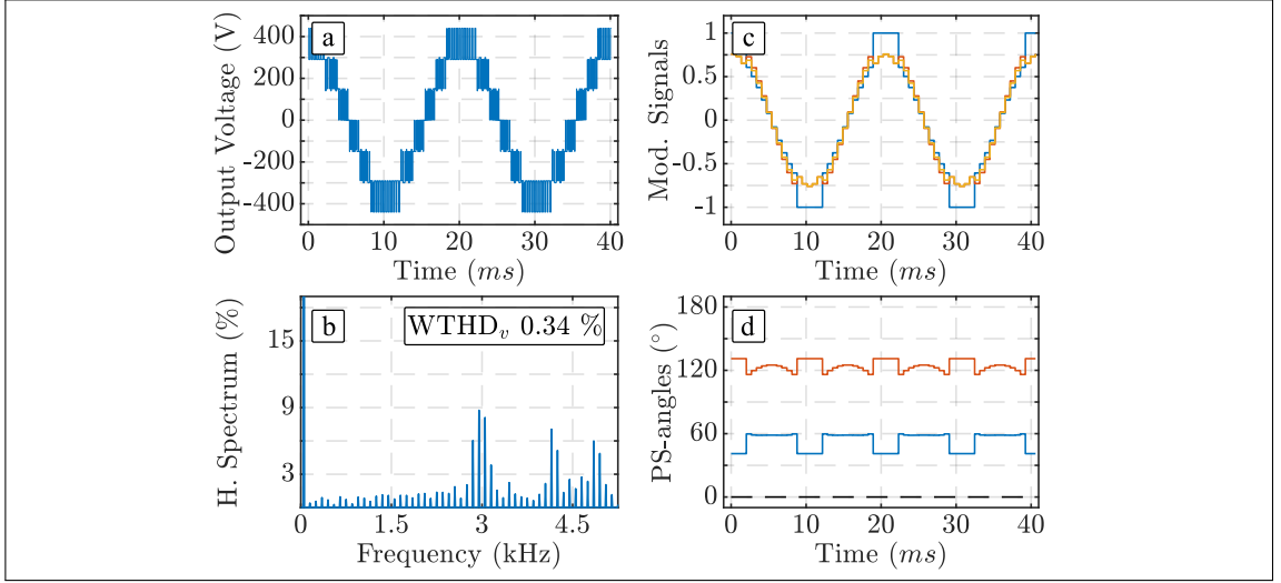
Figure 2.4: Simulation results for the proposed OVA-PS-PWM working as a discontinuous PWM technique. (a) CHB output voltage, (b) voltage harmonic spectra, (c) ac modulating signals, and (d) PS-angles.
