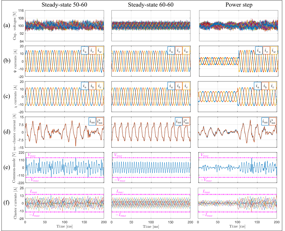
Figure 5.5. Experimental performance in steady-state operating at 50-60 Hz, 60-60 Hz, and a power step at 60-50 Hz. (a) capacitor voltages, (b) input currents, (c) output currents, (d) tracking of ua -cluster current, (e) CMV, and (f) cluster currents.
