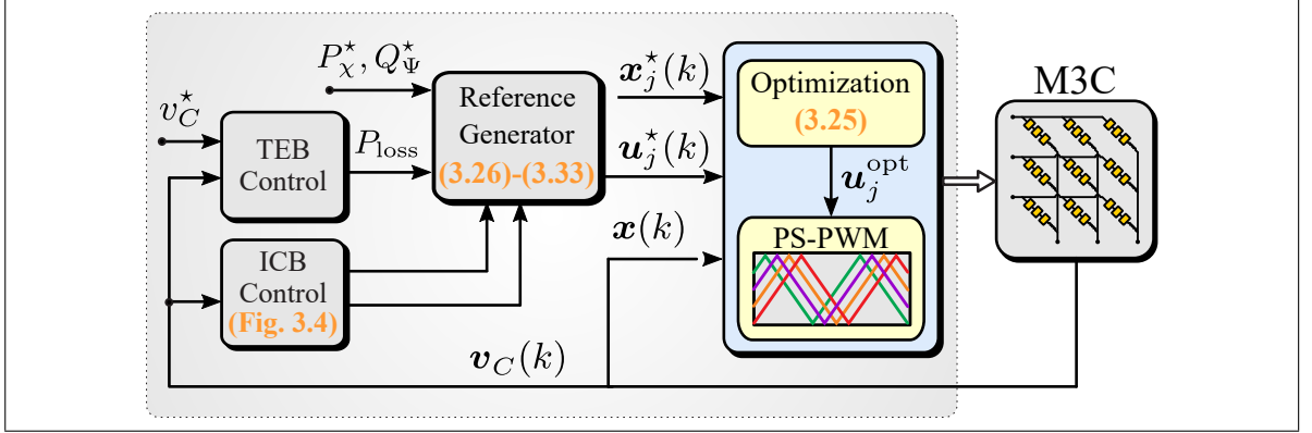
Figure 3.3. Overall control scheme.
