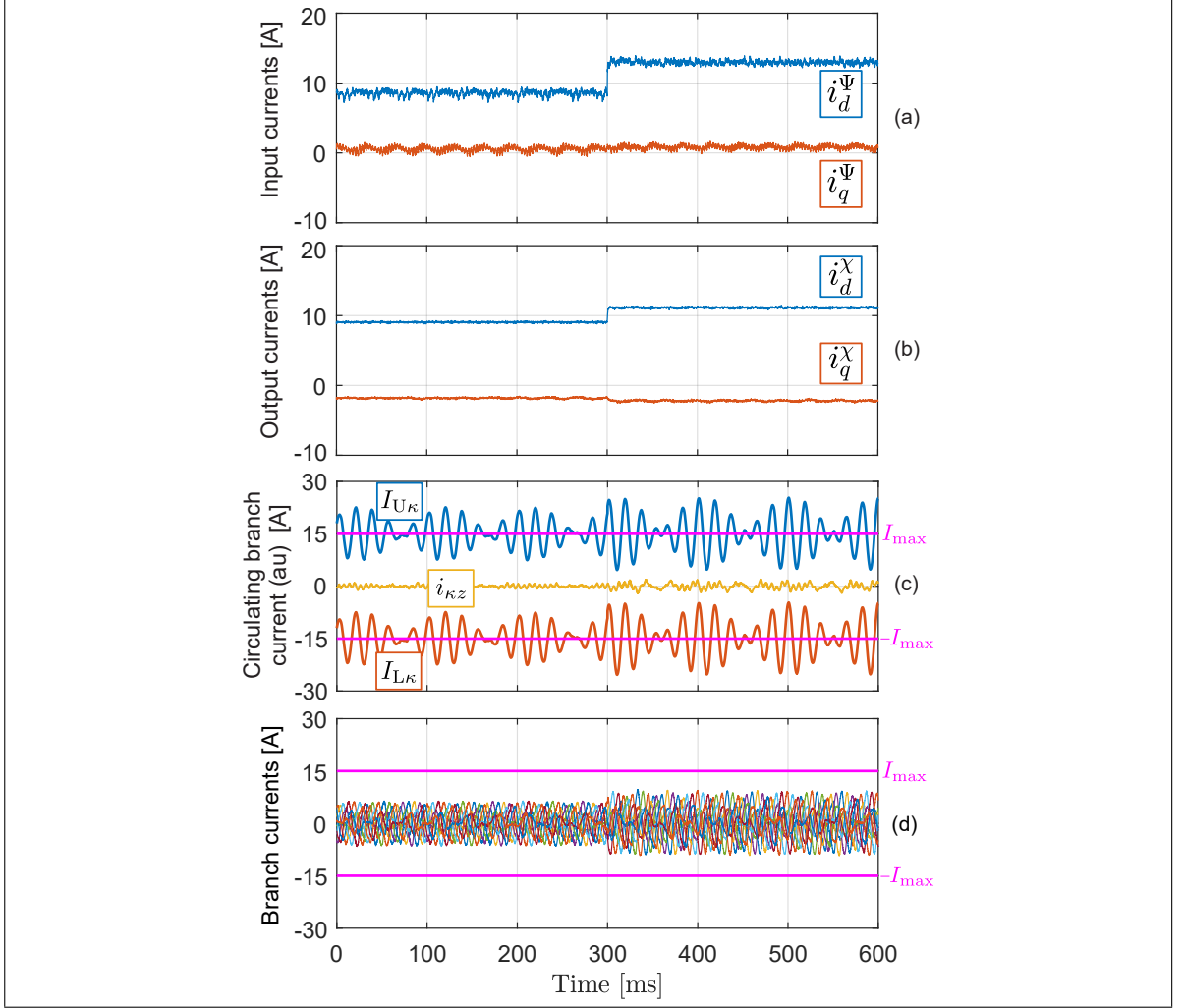
Figure 4.7. Power step performance: input (a) and output (b) currents in rotating dq frames, circulating branch current with their bounds (c), and the total branch currents (d).
