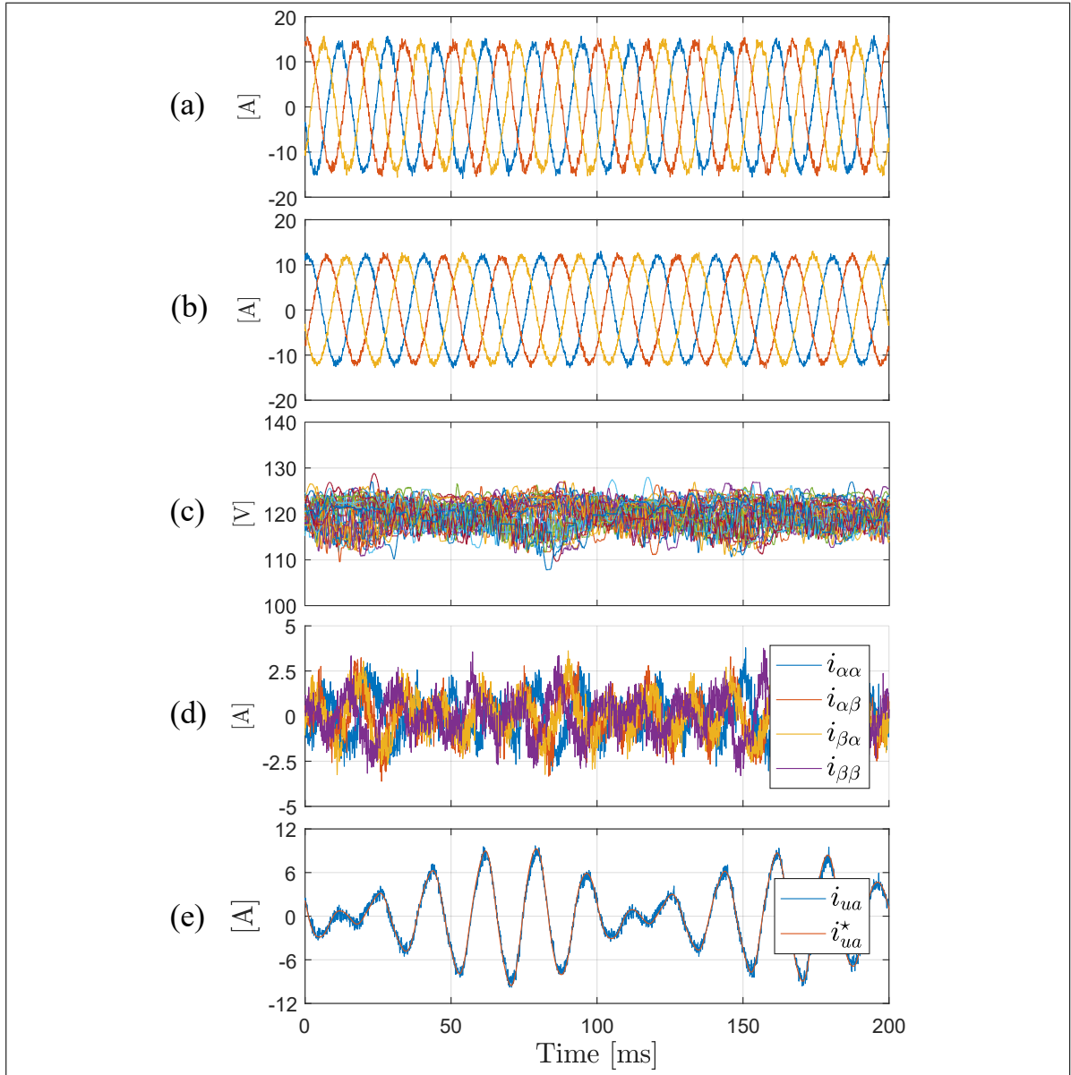
Figure 2.8. Experimental steady-state performance. (a) input currents, (b) output currents, (c) capacitor voltages, (d) circulating currents and (e) u_a -cluster current.
