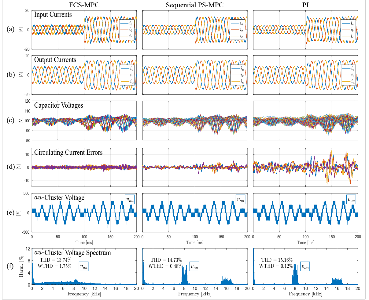
Figure 3.5. Simulation comparison, FCS-MPC strategy (left), the proposed sequential PS-MPC strategy (middle) and PI in dq -framework strategy proposed in (Diaz et al., 2017) (right). (a) input currents, (b) output currents, (c) capacitor voltages, (d) circulating currents tracking error, (e) au -cluster voltage and (f) au -cluster voltage spectra.
