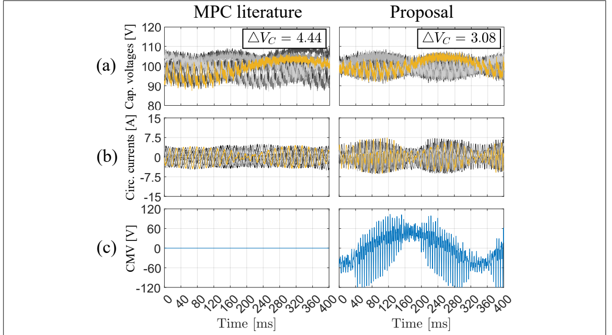
Figure 5.11. Experimental comparison at low frequency 1 Hz.
