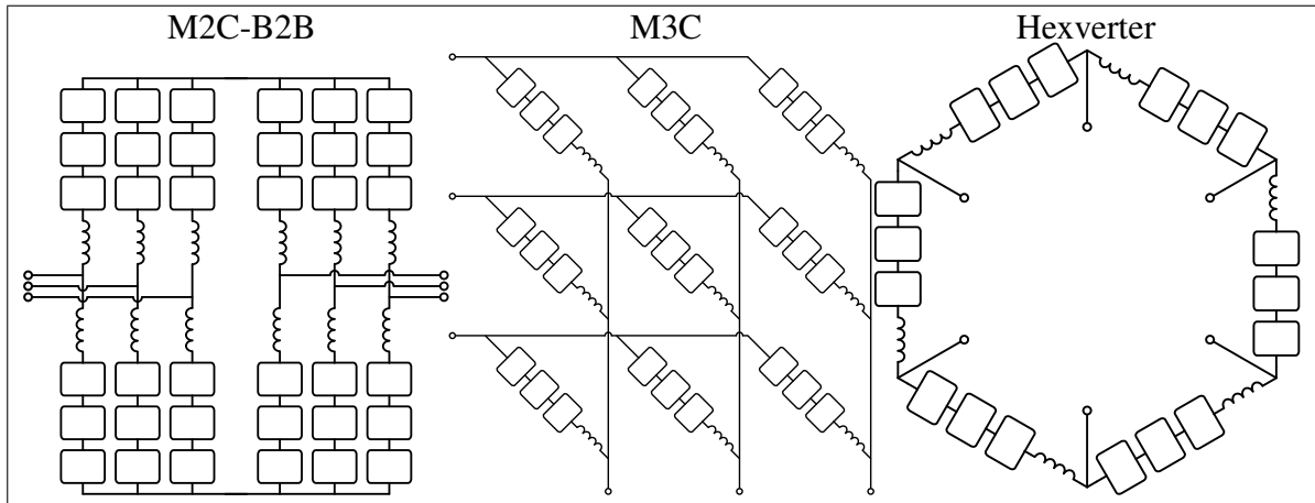
Figure 1.3. Modular multilevel cascaded converters for ac-ac conversion
