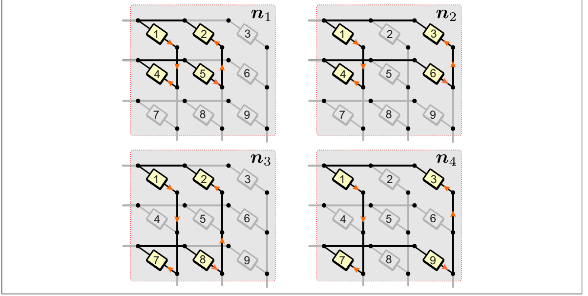
Figure 4.2. Four circulating current paths in the M3C.
