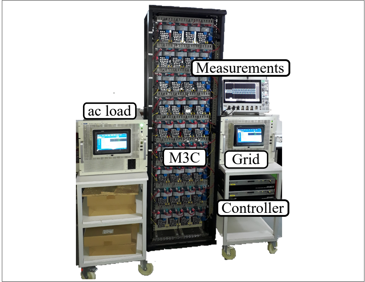
Figure 4.4. Experimental setup with a downscale M3C prototype of 36 SMs.
