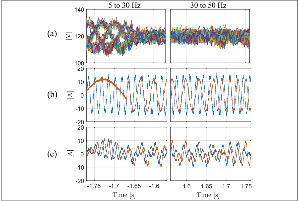
Figure 2.14. Experimental dynamic response under frequency changes. (a) capacitor voltages; (b) input and output current; and (c) ua - and va -cluster current.
