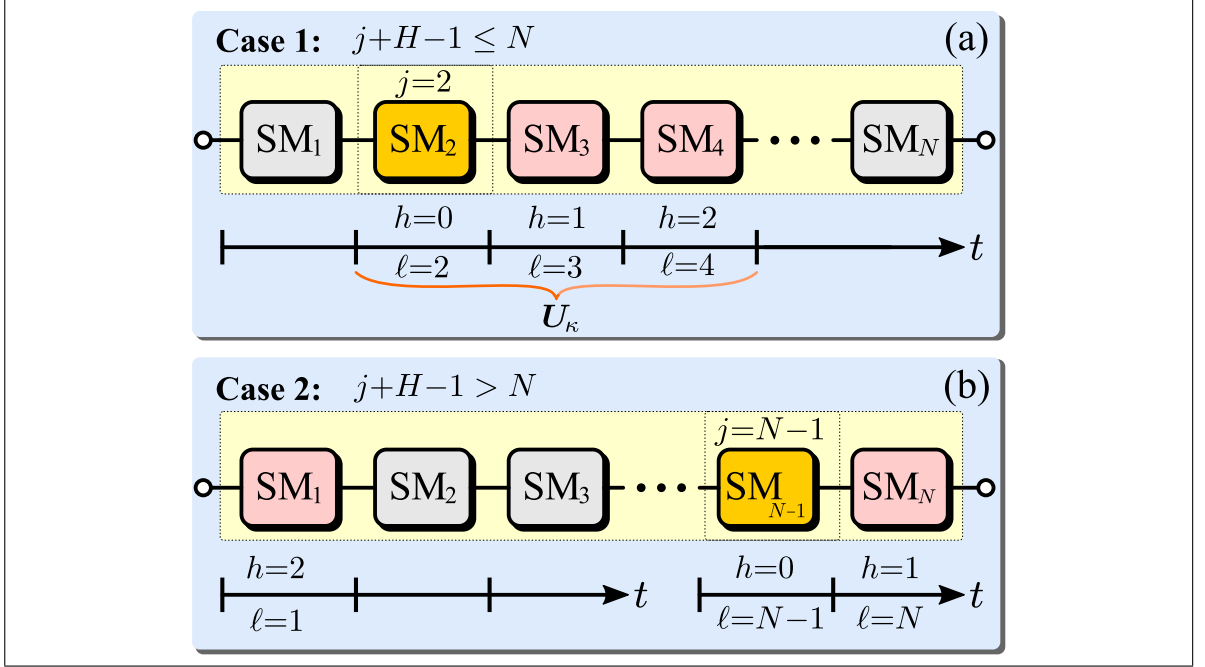
Figure 2.2. Optimization process over horizon length H = 3 : (a) sub-modules to evaluate when j + H - 1 \leq N ; and (b) sub-modules to evaluate and reset when j + H - 1 > N .
