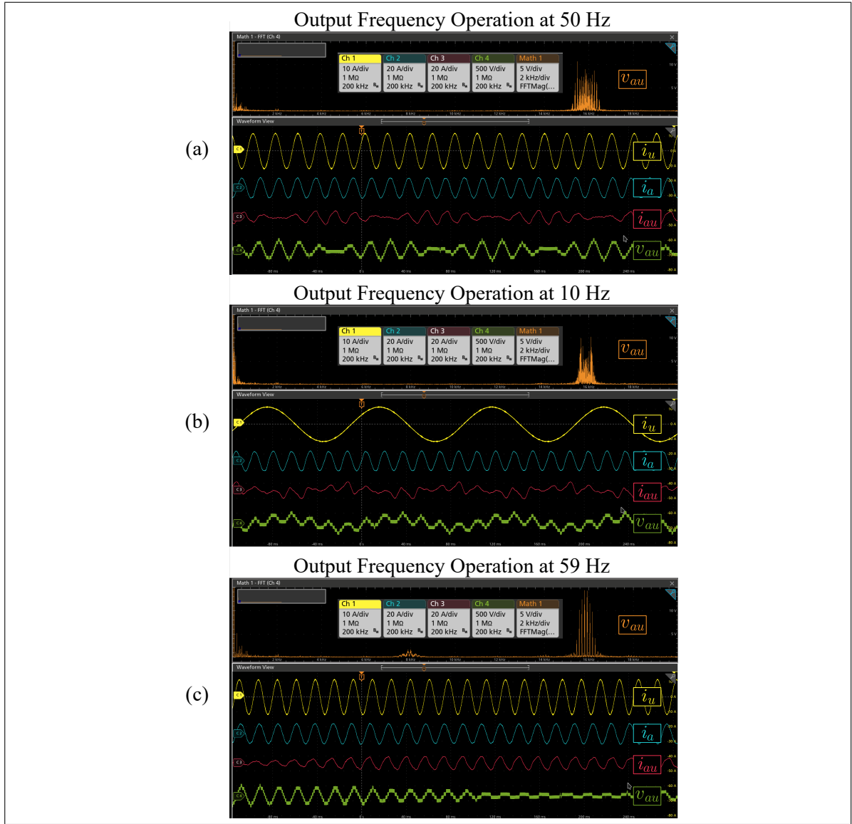
Figure 3.9. Experimental steady-state performance. (Ch 1) output current u , (Ch 2) input current a , (Ch 3) current au -cluster, (Ch 4) output voltage au -cluster, and (Math 1) output voltage au -cluster spectrum. (a) output frequency at 50 Hz, (b) output frequency at 10 Hz, and (c) output frequency at 59 Hz.
