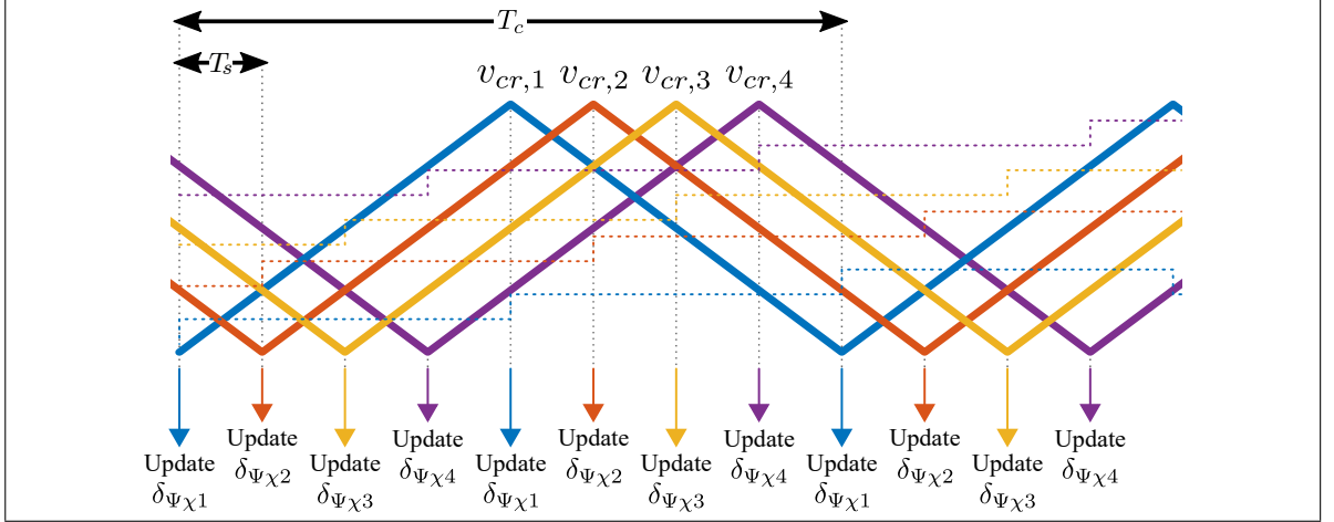
Figure 3.2. PS-PWM operating principle in double update mode for a four-sub-module arm.
