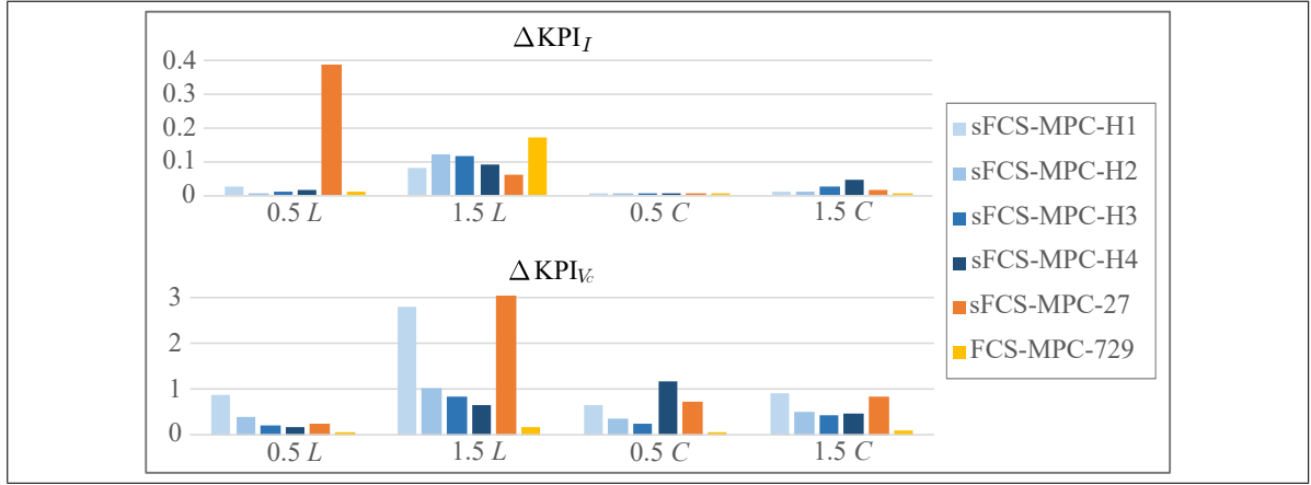
Figure 2.9. Experimental mismatches between control parameters and real hardware values.
