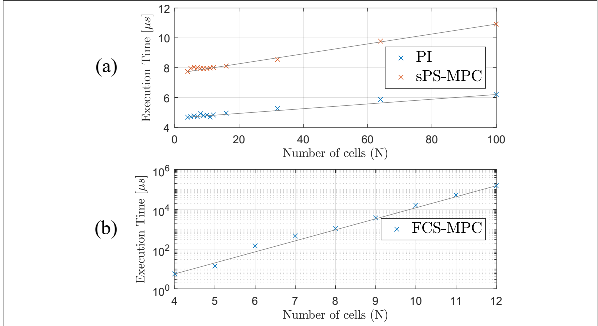
Figure 3.11. Experimental execution time control strategies. (a) PI and sequential PS-MPC strategies and (b) FCS-MPC strategy.
