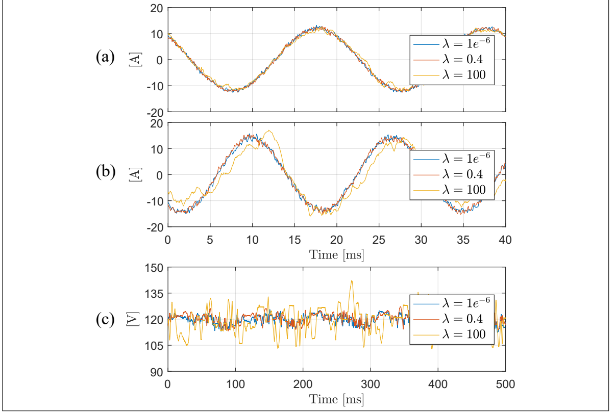
Figure 2.10. Experimental results of the proposal with horizon 4 under different values of \lambda . (a) output-port; (b) input-port; and (c) capacitor voltages.
