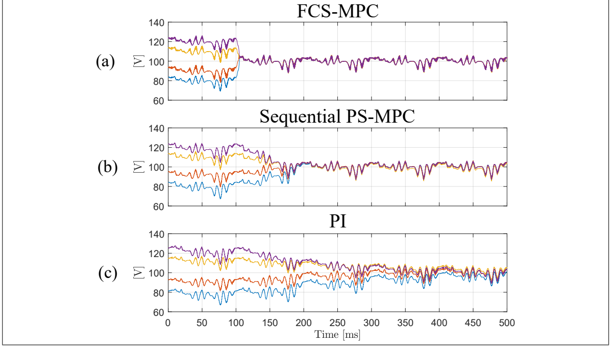
Figure 3.6. Comparison under local-cluster imbalance. Capacitor voltages of au -cluster with (a) FCS-MPC strategy, (b) sequential PS-MPC proposed strategy and (c) PI strategy.
