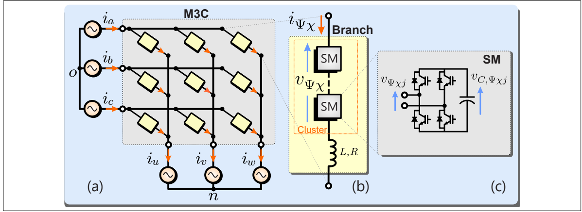
Figure 3.1. The M3C topology: (a) circuit diagram; (b) N -cell cluster; and (c) full-bridge-based submodule.
