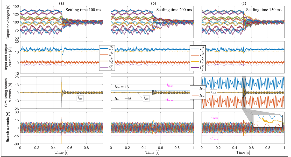
Figure 4.6. Experimental results under imbalance cluster energies: (a) performance of the reference generator introduced in (Urrutia et al., 2022), and performance of the proposed ICB-MPC with static (b) and dynamic (c) upper and lower bounds for i_{kz}^* .
