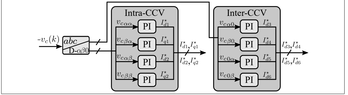
Figure 2.4. Intra-CCV and inter-CCV balancing control (Diaz et al., 2017).
