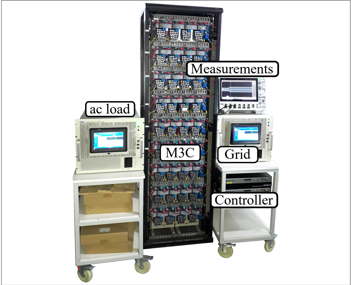
Figure 2.5. 3 kVA experimental prototype.
