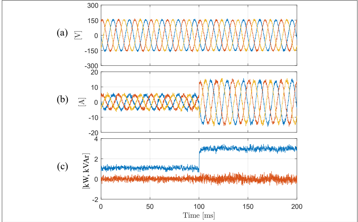
Figure 2.11. Experimental dynamic response of input-port power. (a) input-port voltage; (b) output-port current; and (c) input-port active and reactive power.
