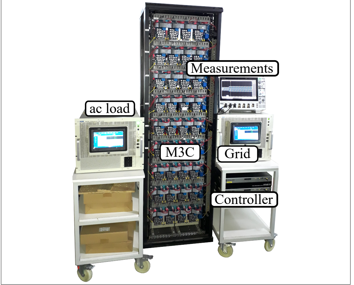
Figure 3.7. 3 kVA experimental prototype
