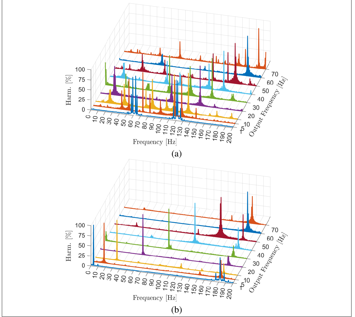
Figure 5.8. Experimental spectrum with output frequency from 1 to 70 Hz. (a) cluster circulating current and (b) CMV.
