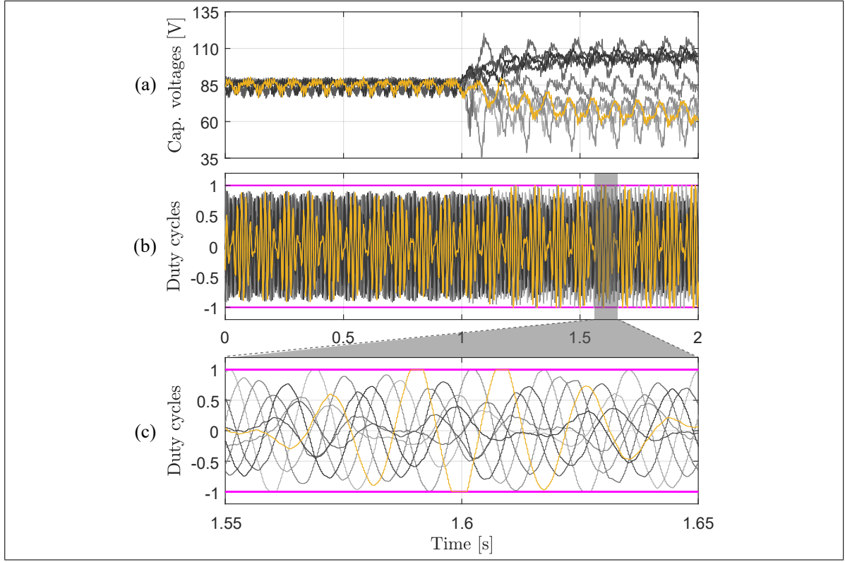
Figure 3.10. Experimental constraints activation under an imbalance condition. (a) capacitor voltages, (b) control signals and (c) control signals zoom.
