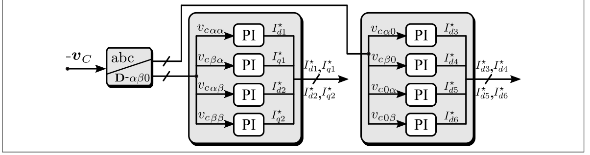
Figure 3.4. Inter-Cluster Balancing control proposed in (Diaz et al., 2017).
