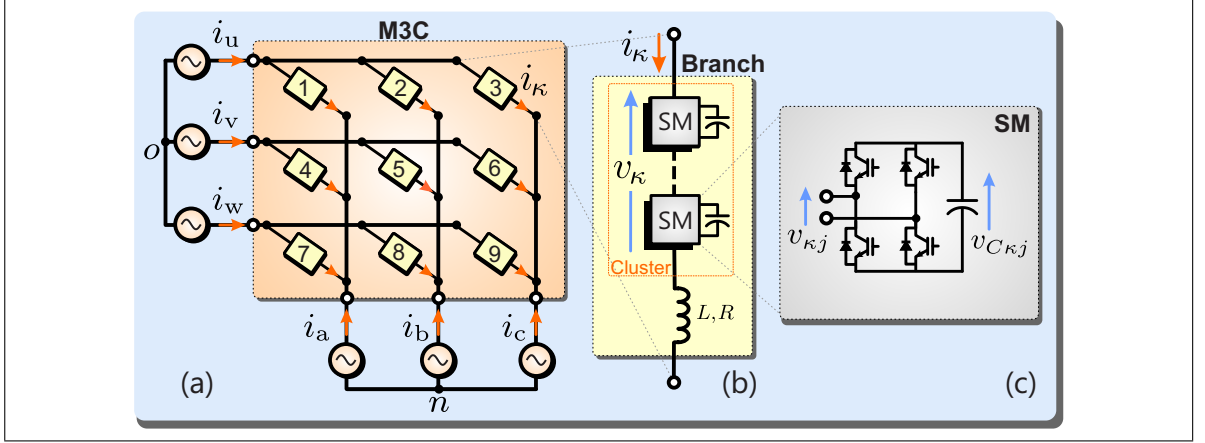
Figure 5.1. The M3C topology: (a) circuit diagram and directed graph; (b) N -cell cluster; and (c) full-bridge-based sub-module.
