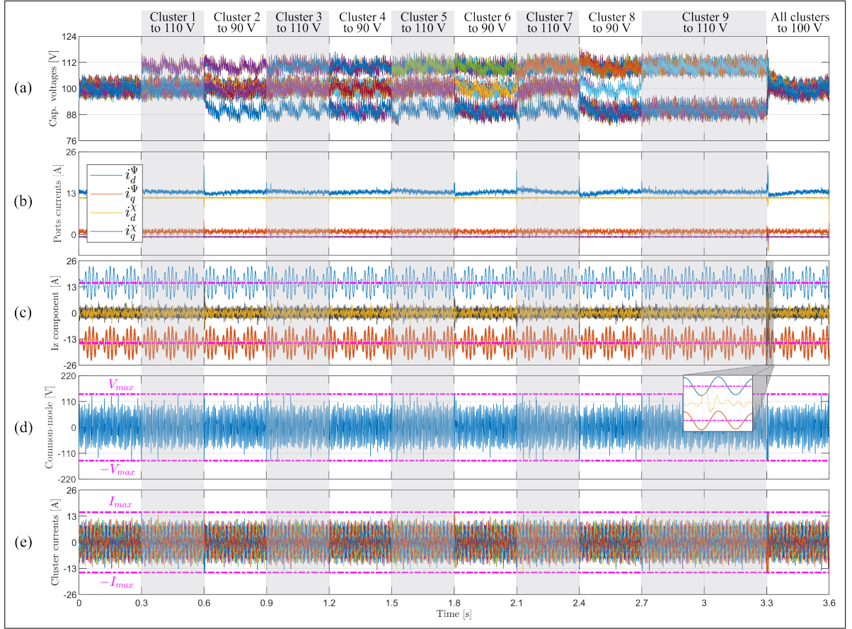
Figure 5.6. Experimental performance under cluster energy imbalance operation. (a) capacitor voltages, (b) input and output currents, (c) circulating current reference with upper and lower bounds of ua -cluster, (d) CMV, and (e) cluster currents.
