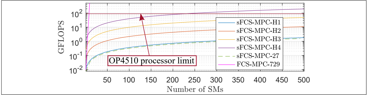
Figure 2.15. FLOPS per control strategy.
