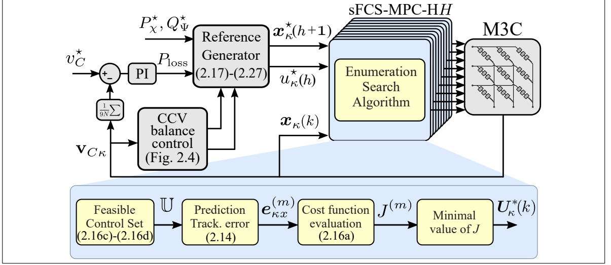
Figure 2.3. Proposed control scheme.
