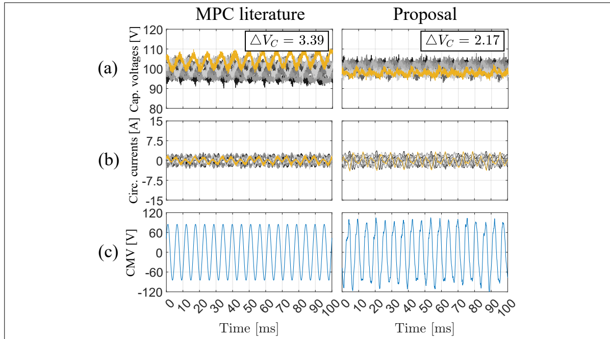
Figure 5.12. Experimental comparison at equal frequency 60 Hz.
