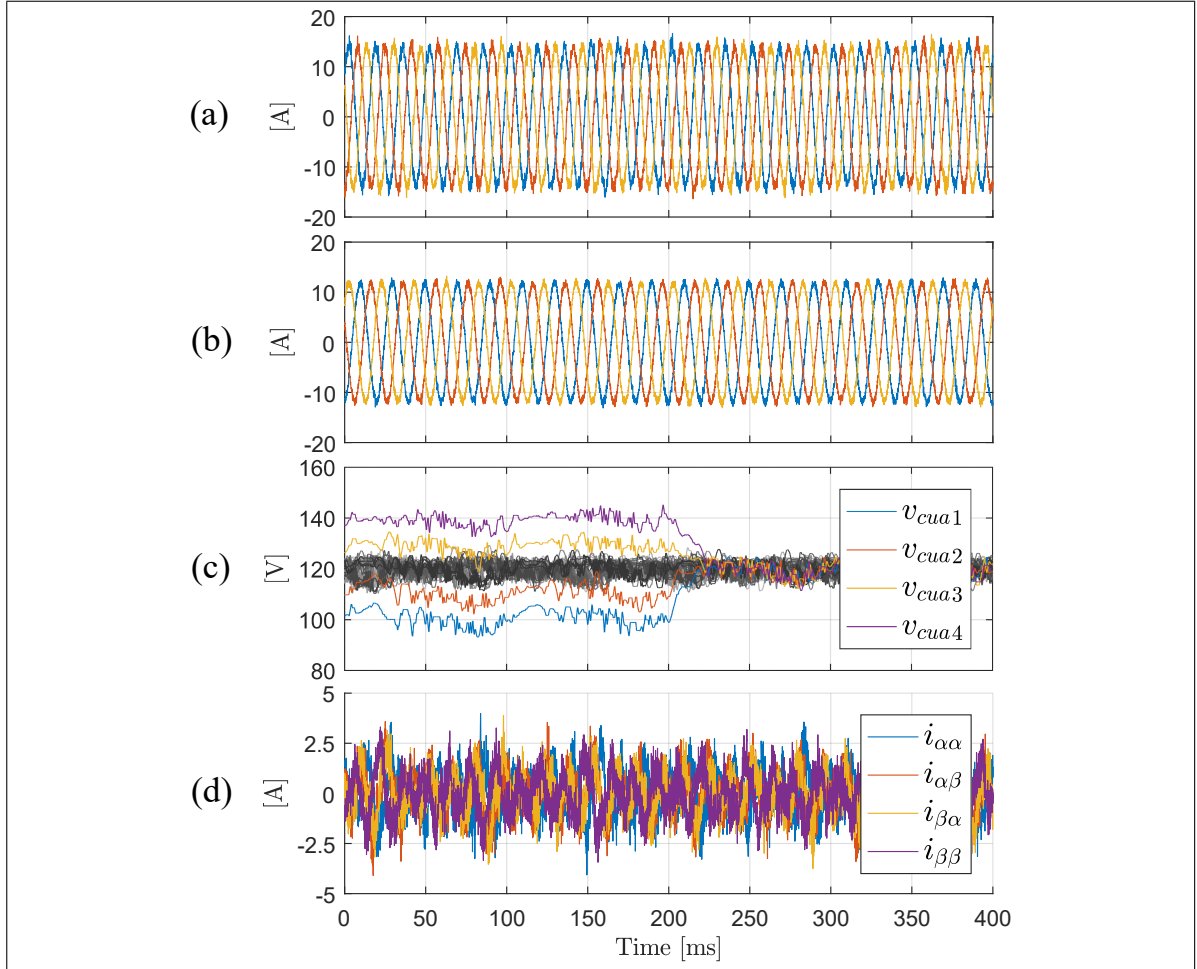
Figure 2.12. Experimental intra-cluster imbalance. (a) input currents, (b) output currents, (c) capacitor voltages, (d) circulating currents.
