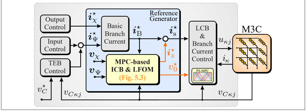
Figure 5.2. Overall control scheme.
