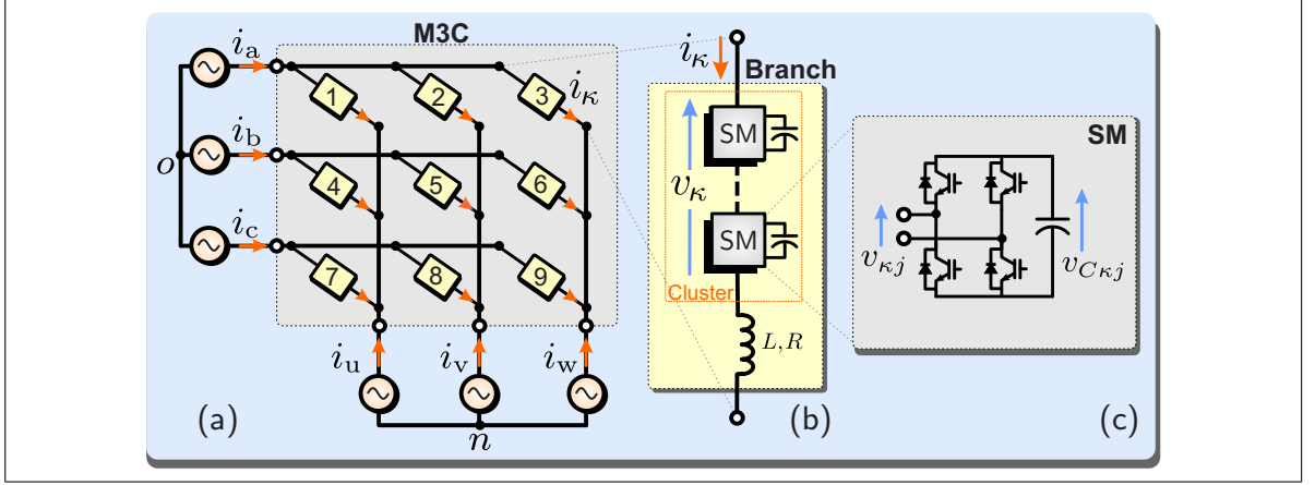
Figure 4.1. The M3C topology: (a) circuit diagram and directed graph; (b) N -cell cluster; and (c) full-bridge-based submodule.
