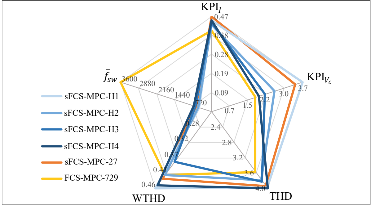
Figure 2.7. Experimental key performance indexes radial graph.
