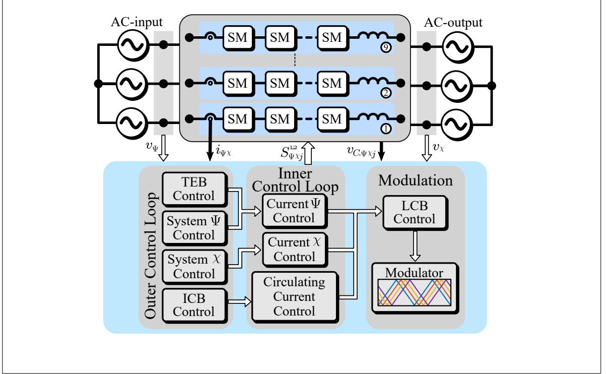
Figure 1.4. General control scheme for the modular multilevel matrix converter
