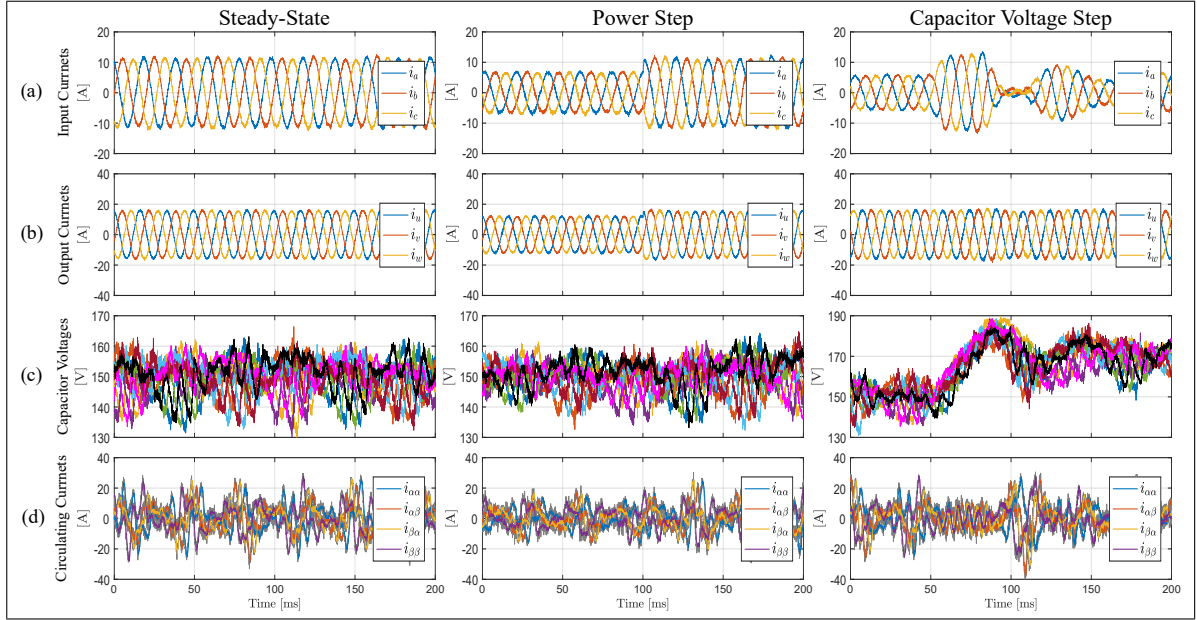
Figure 3.8. Experimental steady-state performance (left), dynamic response performance under a sudden power change (middle) and dynamic response under a sudden capacitor voltage change (right). (a) input currents, (b) output currents, (c) capacitor voltages and (d) circulating current.
