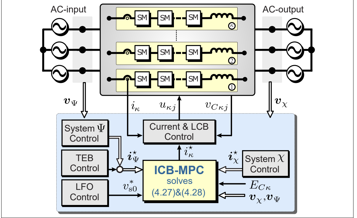
Figure 4.3. Overall control scheme.
