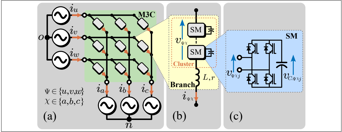
Figure 2.1. The M3C topology: (a) circuit diagram; (b) N -cell cluster; and (c) full-bridge-based sub-module.
