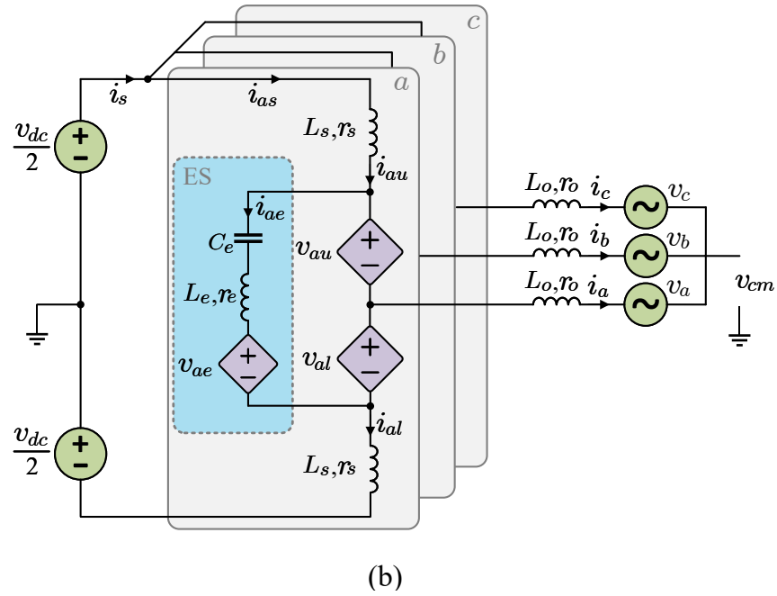
FIGURE 6.2. Proposed MMC with Parallel ES Branches. (a) Configuration with inductors at the ac side. (b) Configuration with the inductors at the dc side.
