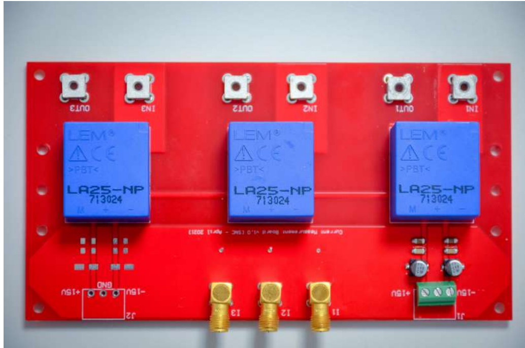
FIGURE 8.5. Designed Current Measurement Board.
