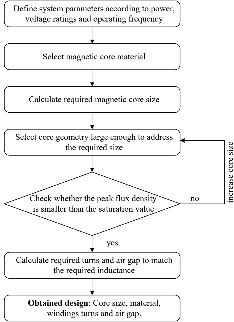
FIGURE 4.6. Flowchart illustrating the coupled inductor magnetic design.
