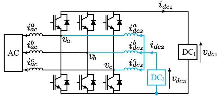
FIGURE 5.6. Three-phase implementation of the TPC.
