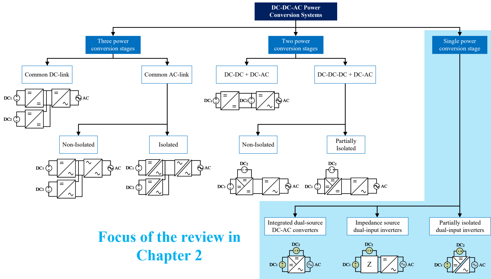
FIGURE 1.6. Classification of DC-DC-AC Power Conversion Systems.
