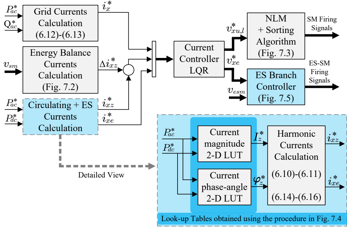
FIGURE 7.1. Overall control scheme.
