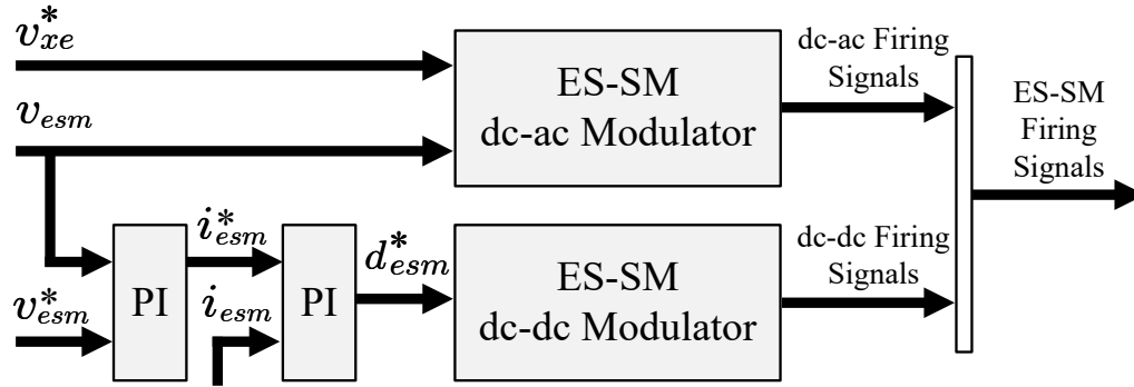
FIGURE 7.5. ES branches control scheme.
