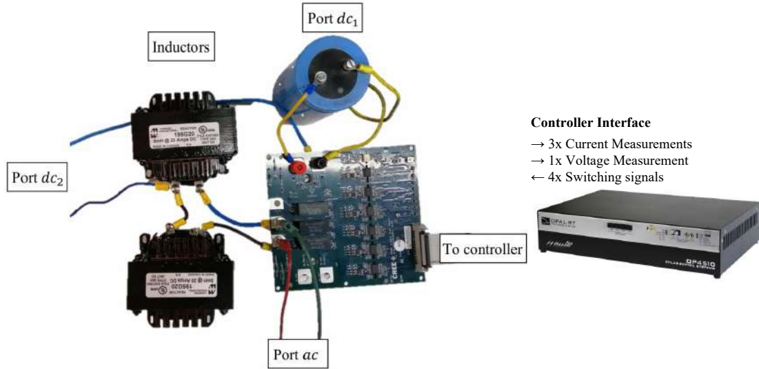
FIGURE 5.12. Experimental TPC cell using CREE CMF20102D.
