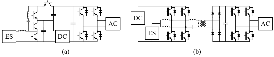
FIGURE 1.10. Examples of a two power conversion stages system with DC-DC-DC + DC-AC converters. (a) Non-Isolated. (b) Partially-Isolated.
