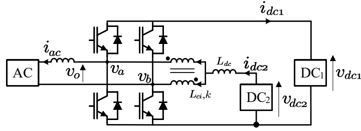
FIGURE 5.8. Single-phase implementation of the TPC with coupled inductors interface.
