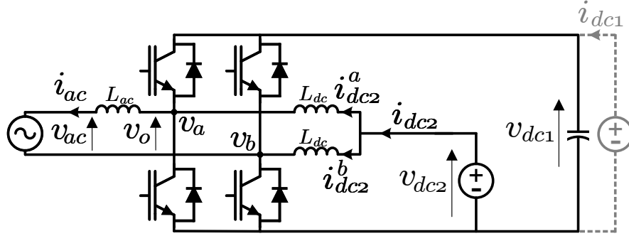
FIGURE 3.4. TPC configuration with energy storage unit on port DC_2 .
